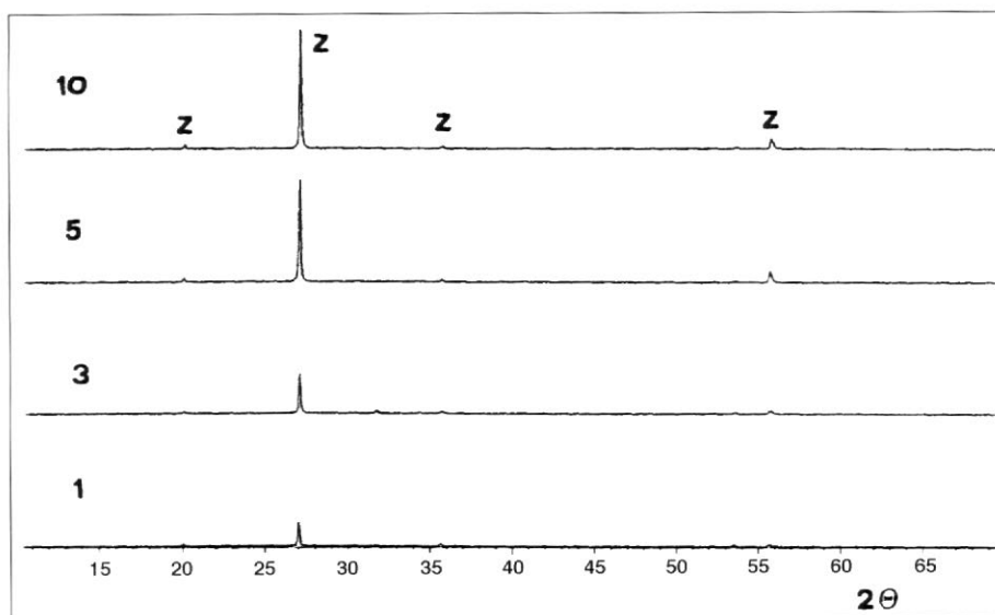
Figure 2. XRD of the cryolite \text{Na}_3\text{AlF}_6 additions to base A: (a)1%,(b)3%,(c)5%,(d)10%.
