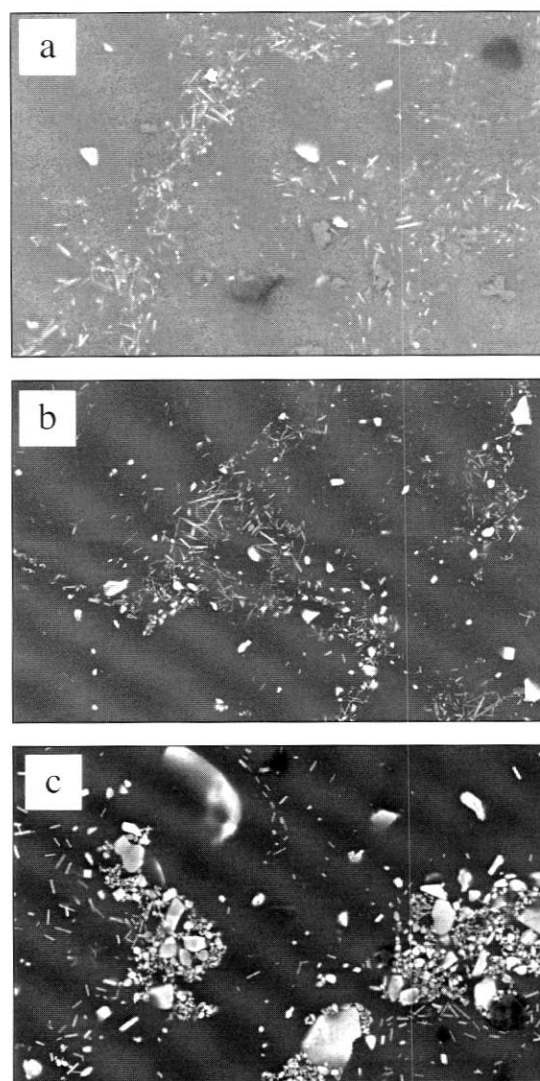
Figure 3. SEM micrographs with back-scattering detector of the cryolite \text{Na}_3\text{AlF}_6 additions to base A: (a)1%,(b)3%,(c)10%.
