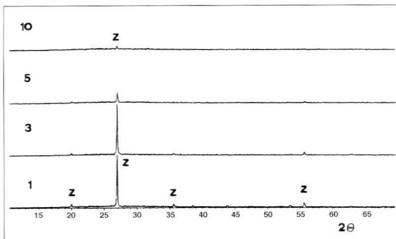
Figure 4. XRD of the \text{Li}_2\text{CO}_3 additions to base A: (a)1%,(b)3%,(c)5%,(d)10%.
