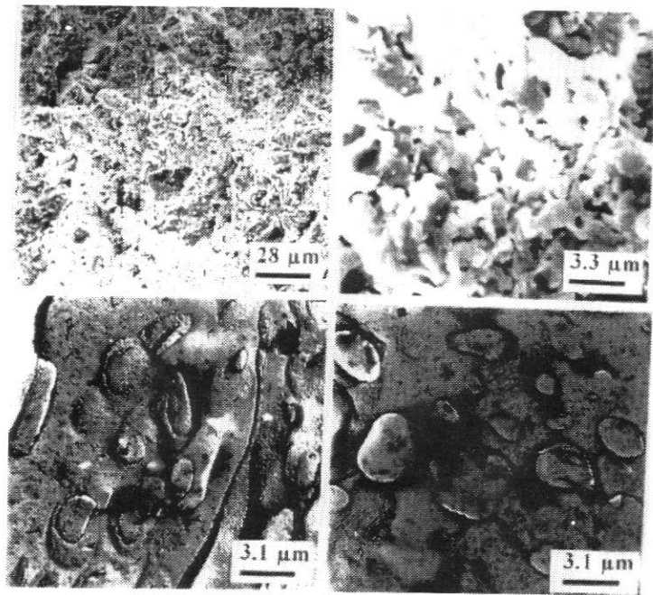
Figure 2.- Electron fractographs obtained from a white, fast-fired substrate: a) and b) SEM and c) and d) TEM
