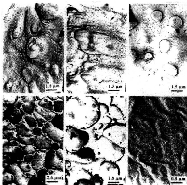
Figure 3.- Several areas observed by transmission electron microscopy (carbon-replica) from a white, fast-fired substrate
