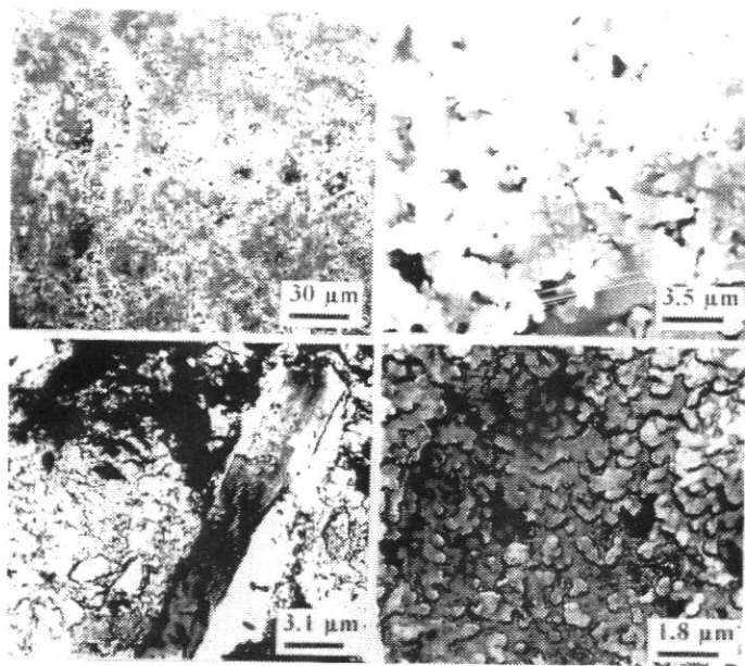
Figure 1.- Electron micrographs from the surface of a white, fast-fired substrate: a) and b) SEM and c) and d) TEM
