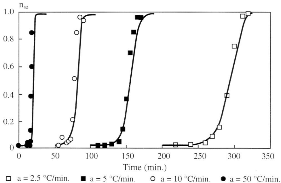
Figure 7. Plot of the experimental data (points) and values calculated from Eqs. (6) and (7) (solid lines), for each studied heating rate.
