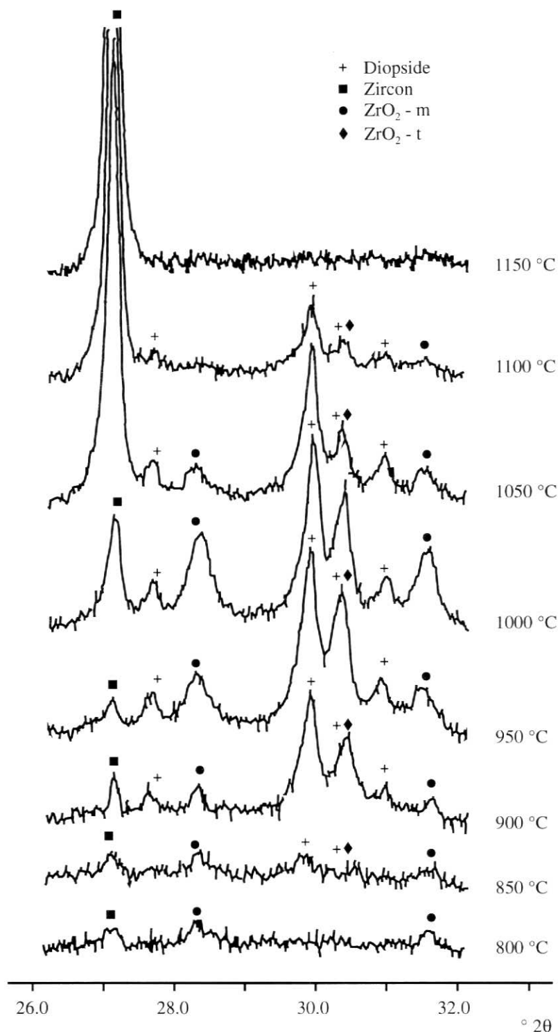
Figure 6. Crystalline phases identified at different peak temperatures. Heating rate 5 °C/min.
