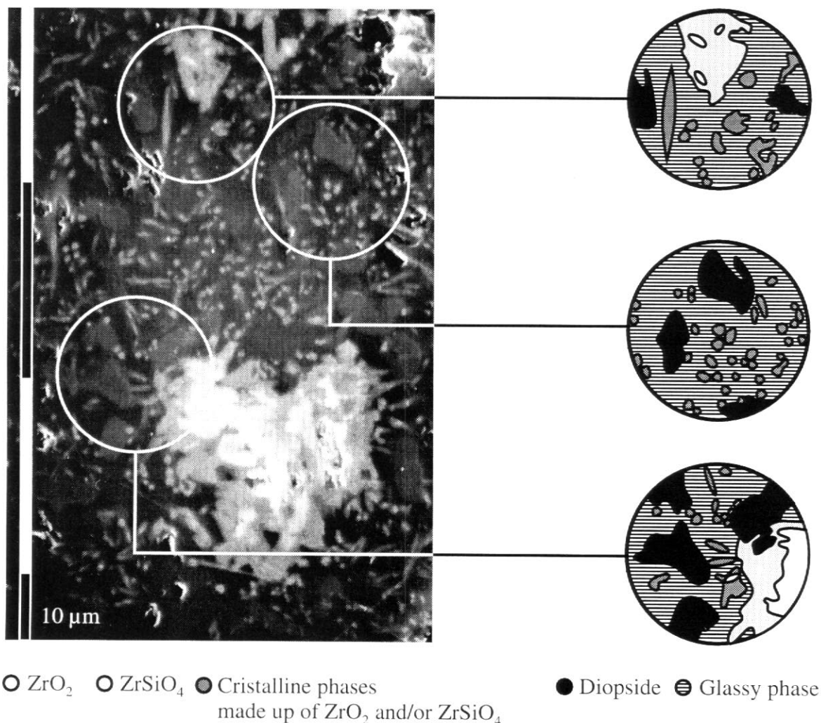
Figure 5. Nature of the devitrifying crystalline phases
