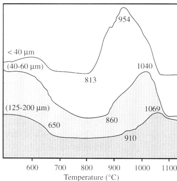
Figure 3. DTA curves corresponding to fractions D_p < 40\mu\text{m} , 40 < D_p < 60\mu\text{m} and 125 < D_p < 200\mu\text{m} of the frit. Heating rate 10^\circ\text{C}/\text{min} .
