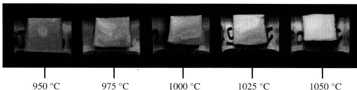
Figure 9. Evolution of the appearance of the test specimens obtained on treating them to different peak temperatures, using a heating rate of 50^\circ\text{C}/\text{min} .
