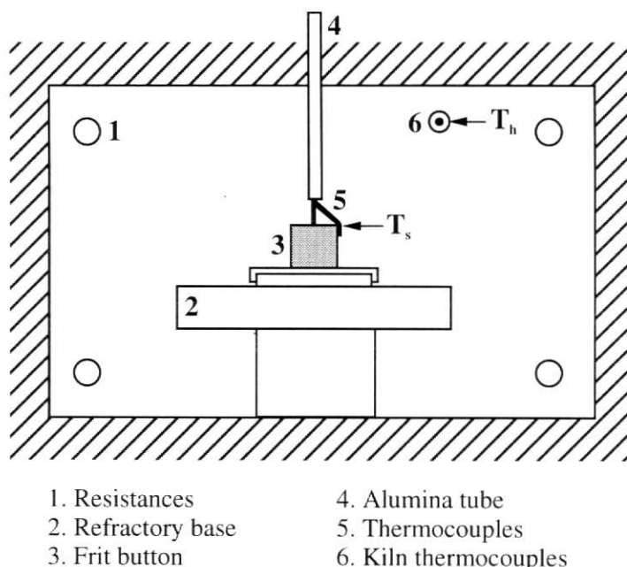
Figure 2. Setup used for determining the variation of T_h , T_s and T_i .
