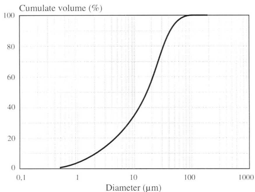
Figure 1. Particle-size distribution of the frit used for preparing the test specimens.
