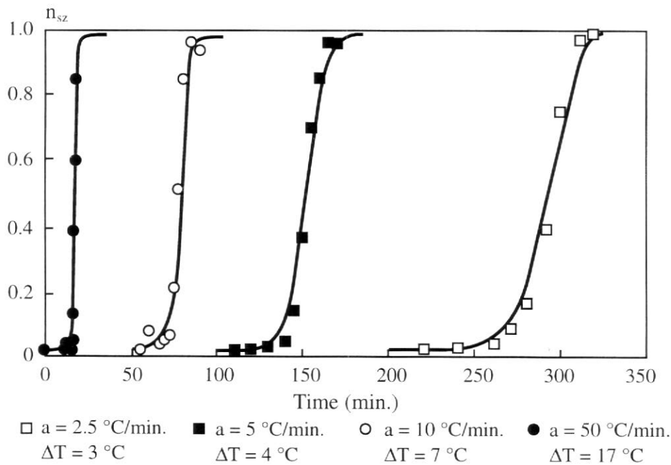
Figure 8. Plot of the experimental data (points) and values calculated using Eqs. (9) and (10) (solid lines), for each tested heating rate.
