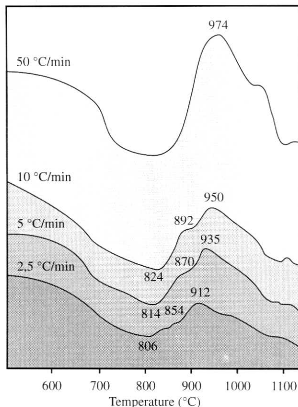
Figure 4. DTA thermograms obtained, corresponding to different heating rates
