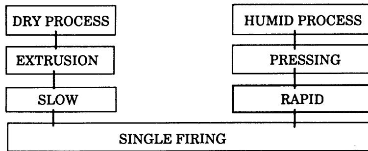
Figure 1. Vitrified paving.
