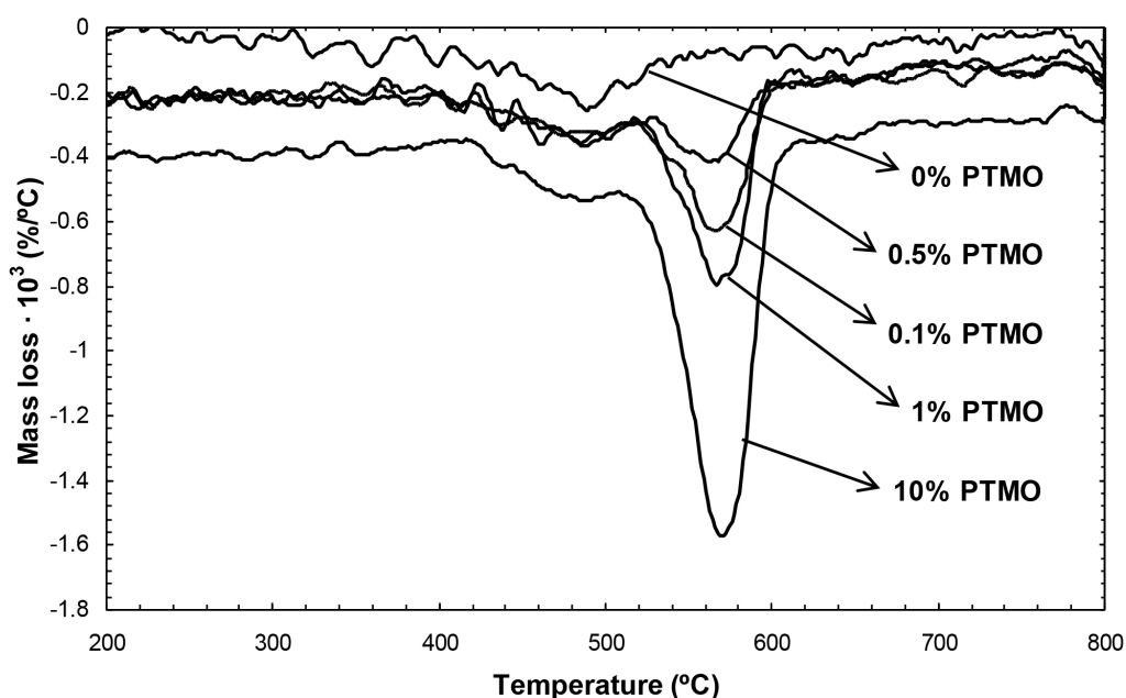
Figure 1. Influence of the proportioned quantity of PTMO on the mass losses of the treated quartz. A reaction time of 3 h was used in every case.
