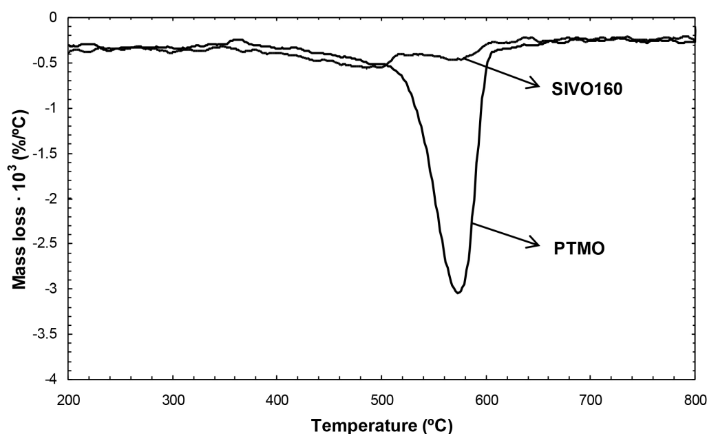
Figure 3. Comparison of the mass losses of quartz treated with PTMO and SIVO160. In both cases, the proportioned quantity was 10% by weight and the reaction time was 5 h.
