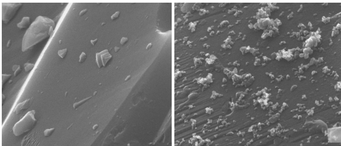
Figure 6. Morphology of the quartz particle surface before (left) and after (right) treatment with 1.5% nano-alumina by weight.
