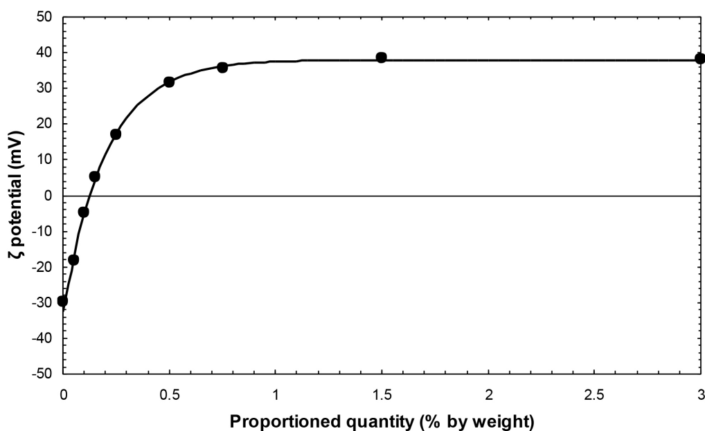
Figure 4. Variation of the \zeta potential of a quartz suspension treated with different proportioned quantities of SIVO160.
