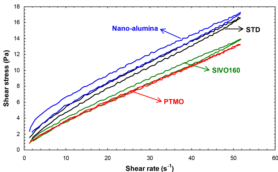
Figure 7. Flow curves of the vitreous china sanitary ware suspension incorporating quartz treatment with different additives.
