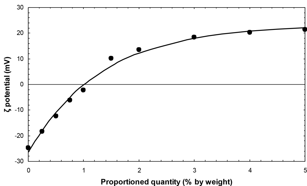
Figure 5. Variation of the \zeta potential of a quartz suspension treated with different proportioned quantities of nano-alumina.
