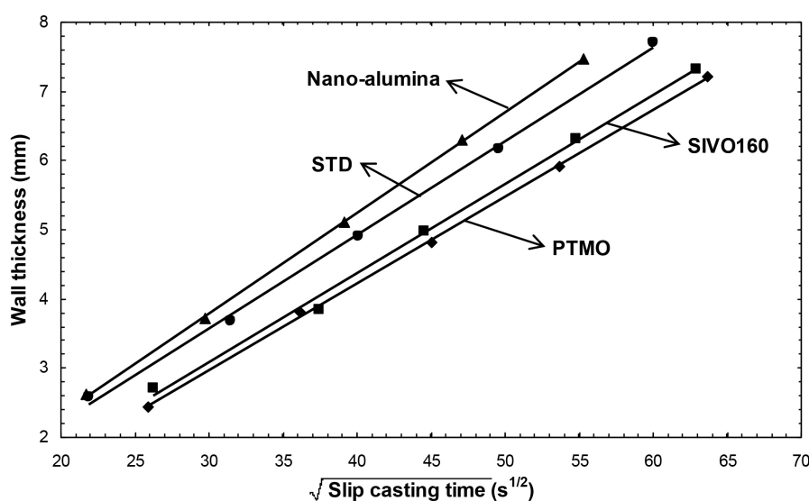
Figure 8. Slip casting kinetics of the sanitary ware composition after treatment with the additives indicated.
