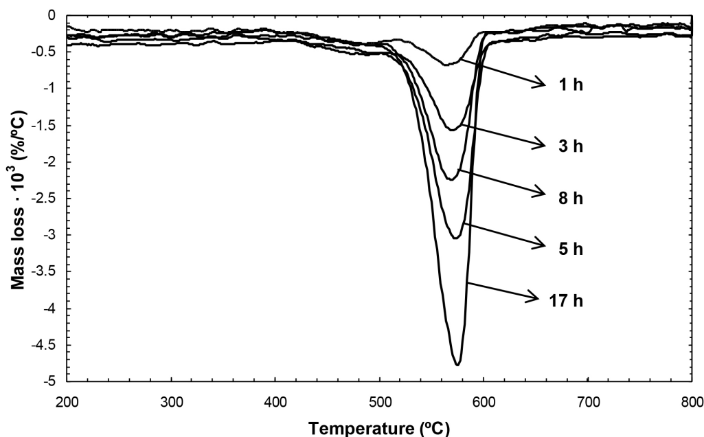
Figure 2. Influence of reaction time on the mass losses of quartz treated with PTMO. The proportioned quantity of PTMO was 10% in every case.
