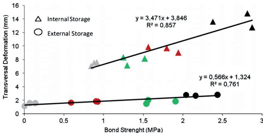
Figure 4. Graph comparing transverse deformation and bond strength of laboratory and exterior in-service samples at 180 day age [6]; note significant reduction in deformation of exterior samples.
