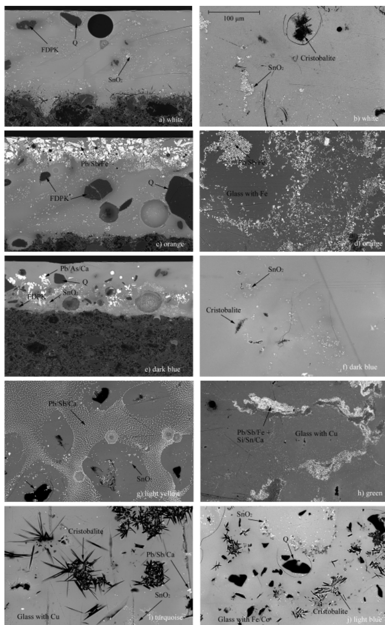
Figure 2. Surface and cross-section of glazes with different colours in the pieces from the 18 th century.
