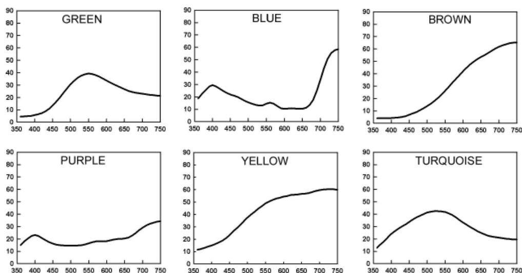
Figure 3, Spectrophotometric curves of the glazes in piece 3 (18 th century). Reflectance in % versus wavelength in nm
