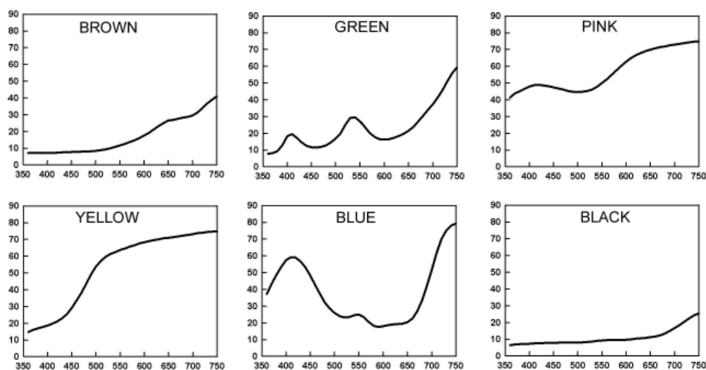
Figure 4. Spectrophotometric curves of the glazes obtained by applying the pure inks. Reflectance in % versus wavelength in nm
