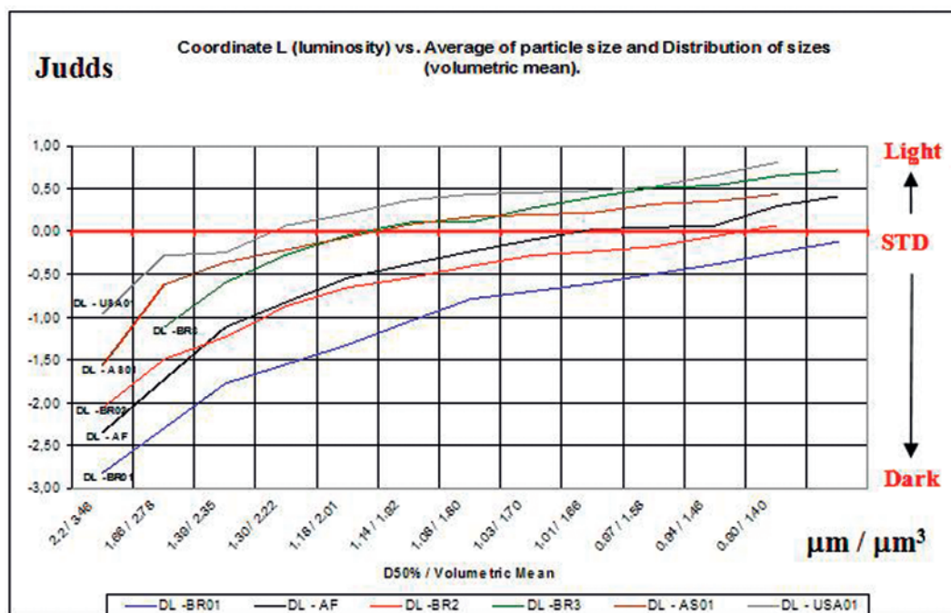
Figure 1. Coordinate L^* vs. average of particle size (D50%) and volumetric mean (M.V.) of 06 zircons compared to a commercial standard.
