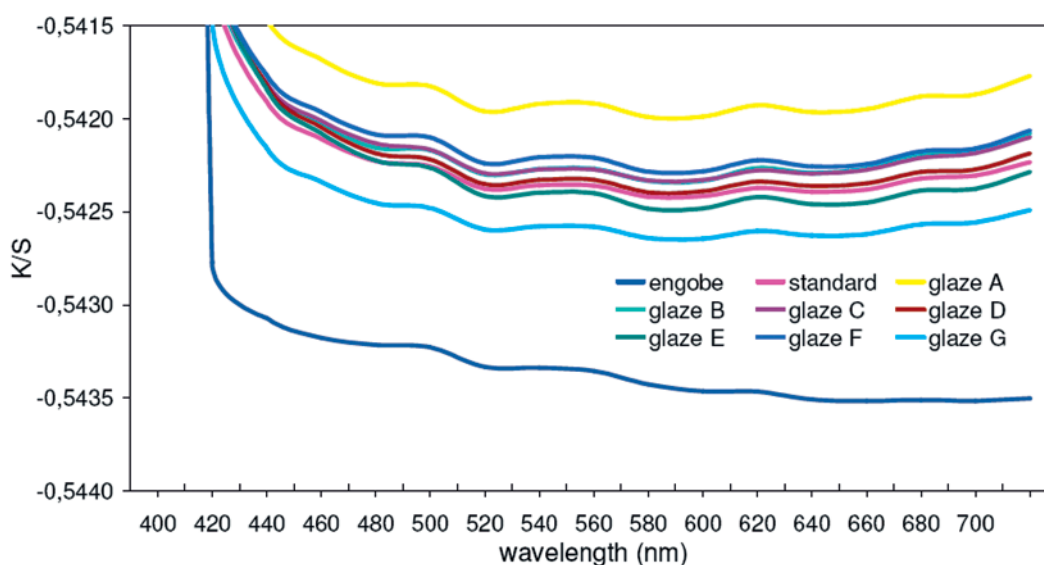
Figure 2. K/S ratio spectra for engobe, standard glaze and test glazes
