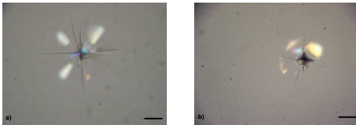
Figure 5. Light micrographs of Vickers indentations and the corresponding crack path of a) S-L G and, b) Red samples in air environment. The bar is 50 \mu\text{m} .
