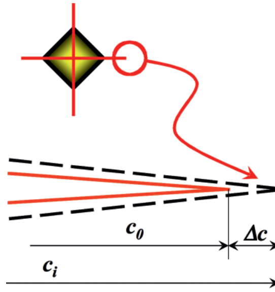
Figure 4. SCG in terms of \Delta c_i = (c_i - c_0) , referred to a single median-radial crack.
