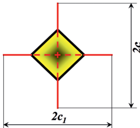
Figure 3. Vickers impression and median-radial cracks.
