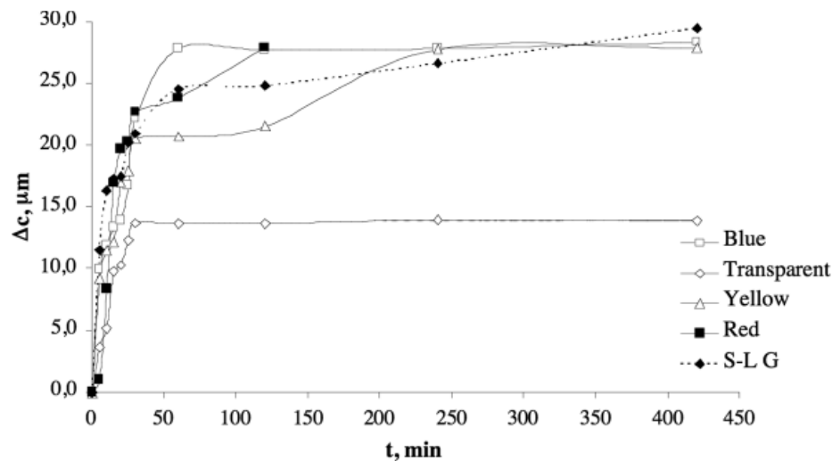
Figure 6. \Delta c_m as function of time, for the tested samples in a) air, b) water and, c) in alkaline solution, KOH 100g/l.
