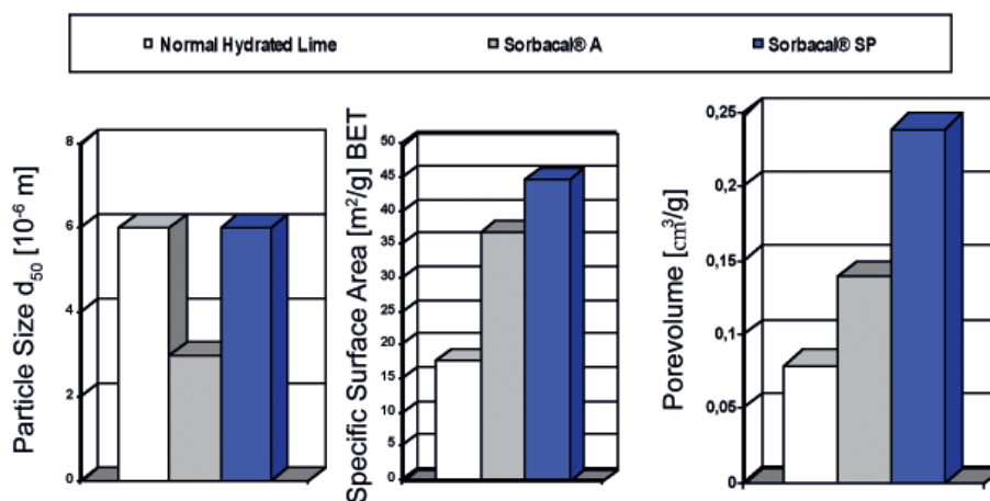
Figure 3. Comparison of different Hydrated Limes
