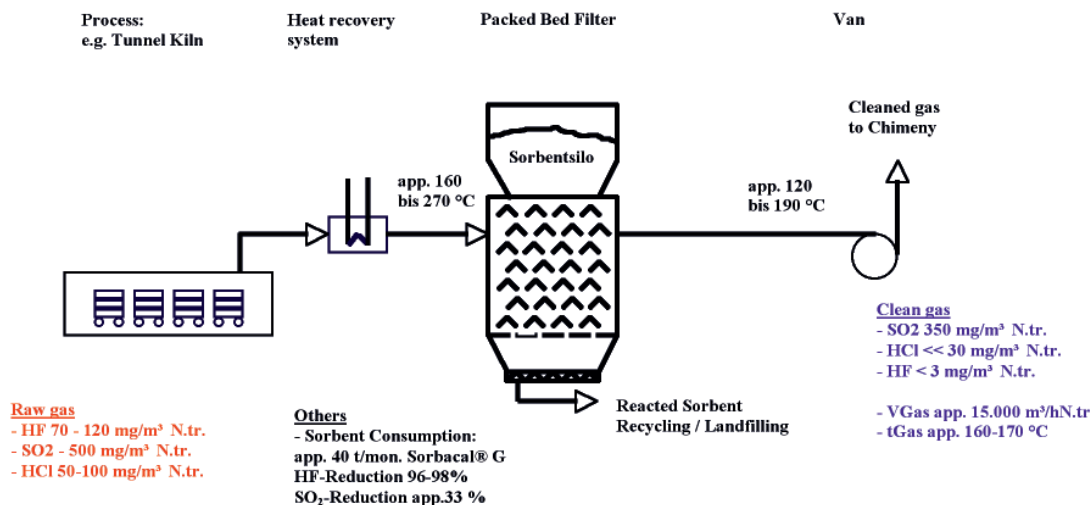
Figure 8. Conventional packed bed filter with granulated sorbent
