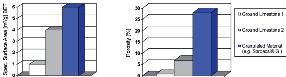
Figure 5. Specific surface area and porosity of ground limestone and granulated sorbent
