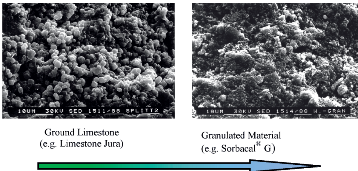
Figure 6. Scanning electron microscope pictures of ground limestone and granulated sorbent
