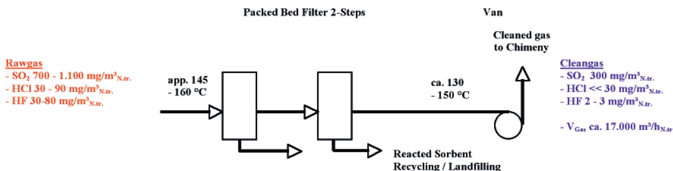
Figure 9. Multistage packed bed filter systems (2-stage)
