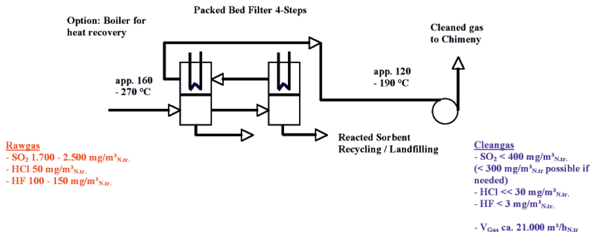
Figure 10. 4-stage packed bed filter system with temperature management
