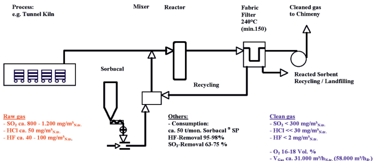
Figure 11. Dry sorption with fabric filter
