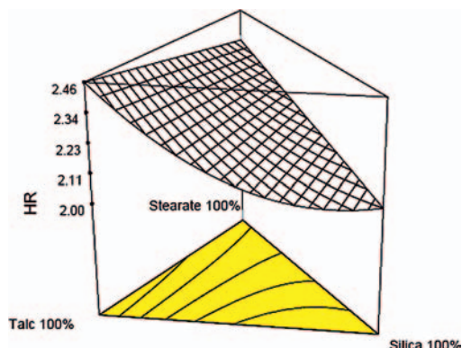
Figure 2. 3D response surface for yellow pigment
