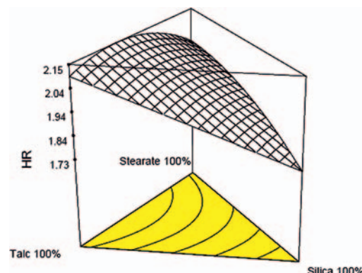
Figure 3. 3D response surface for black pigment
