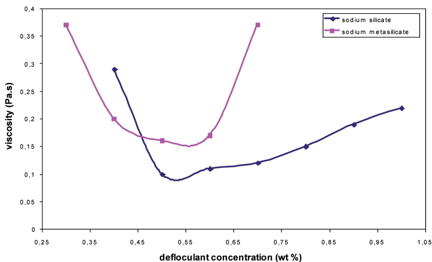
Figure 2. Viscosity curves for the ceramic suspension in function of the type of deflocculant used
