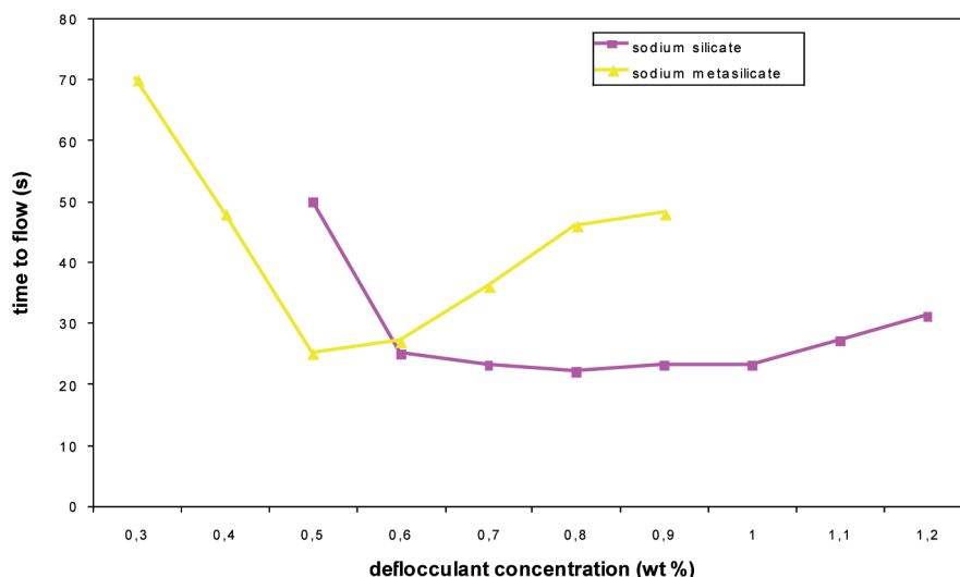
Figure 1. Flow curves for the ceramic suspension in function of the type of deflocculant used
