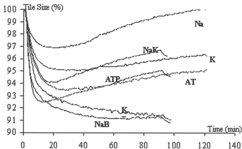
Figure 9: Isothermal curves at 1200°C for the different porcelain stoneware bodies.
