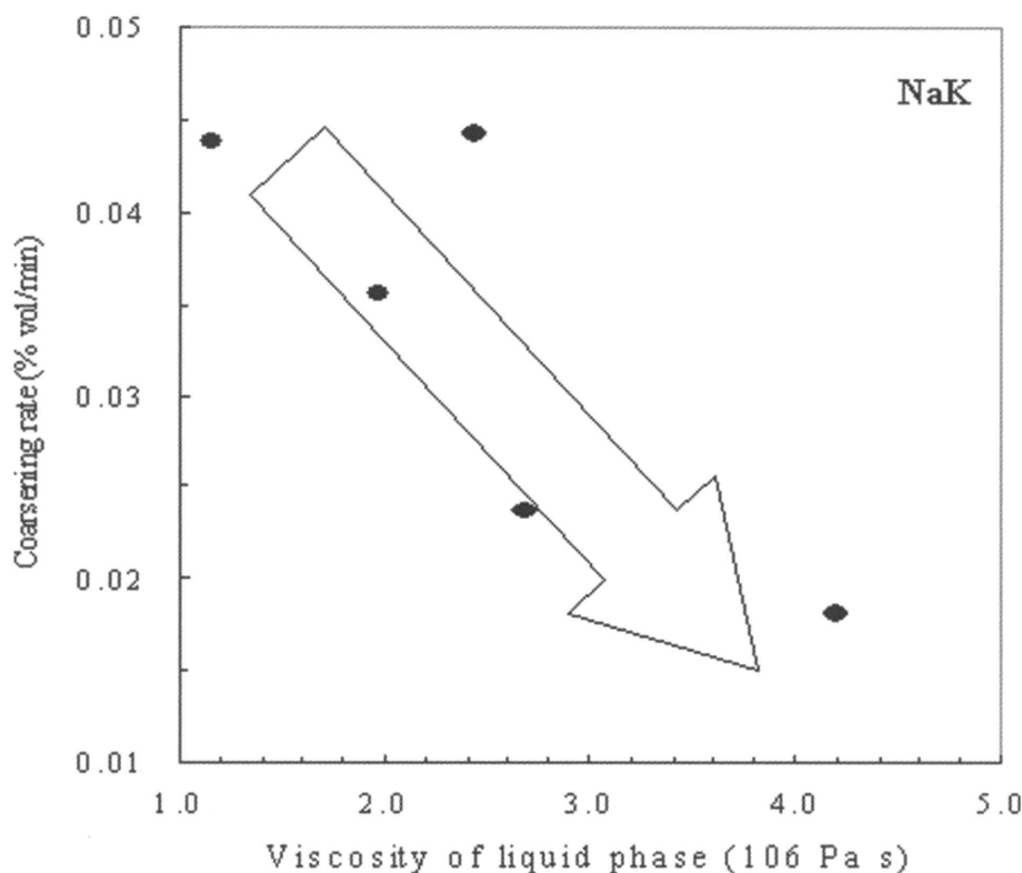
Figure 13: Correlation between the viscosity of the liquid phase and the coarsening rate of porcelain stoneware (body NaK).
