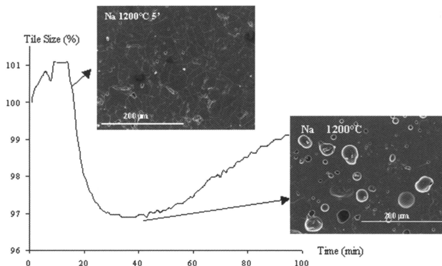
Figure 11: Example of coarsening during the isothermal sintering (1200°C) of porcelain stoneware (body Na).
