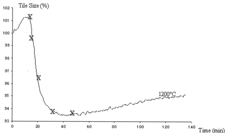
Figure 2: Isothermal (1200°C) densification curve for the industrial sample AT. The X symbols indicate the times of progressive densification at which quenching was done.
