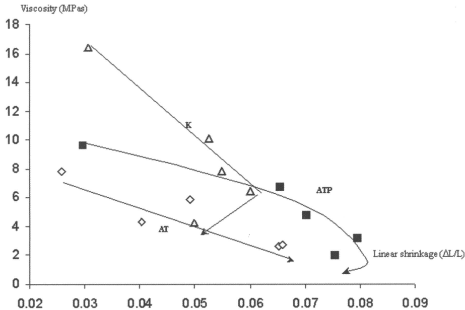
Figure 7: Relationship between linear shrinkage and viscosity of the liquid phase for samples ATP, AT and K.
