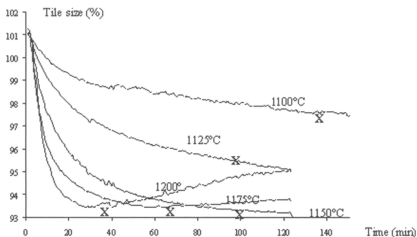
Figure 1: Isothermal densification curves for the industrial sample AT. The X symbols indicate for each temperature the time of maximum densification at which quenching was done.
