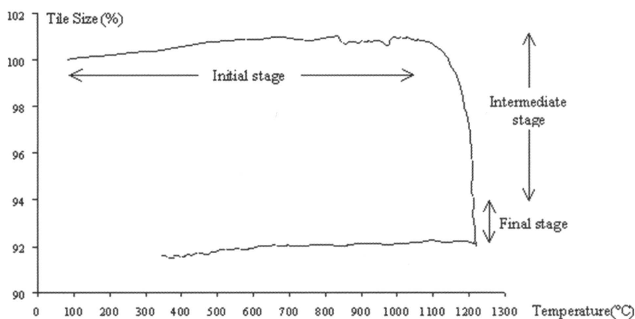
Figure 3: Example of constant rate sintering curve of an industrial sample of porcelain stoneware tile.
