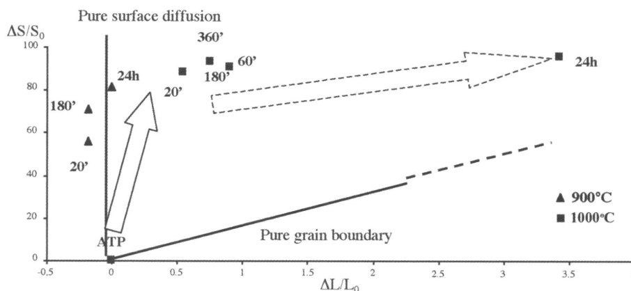
Figure 4: Relationship between linear shrinkage ( \Delta L/L_0 ) and reduction of specific surface area ( \Delta S/S_0 ) [13] .
