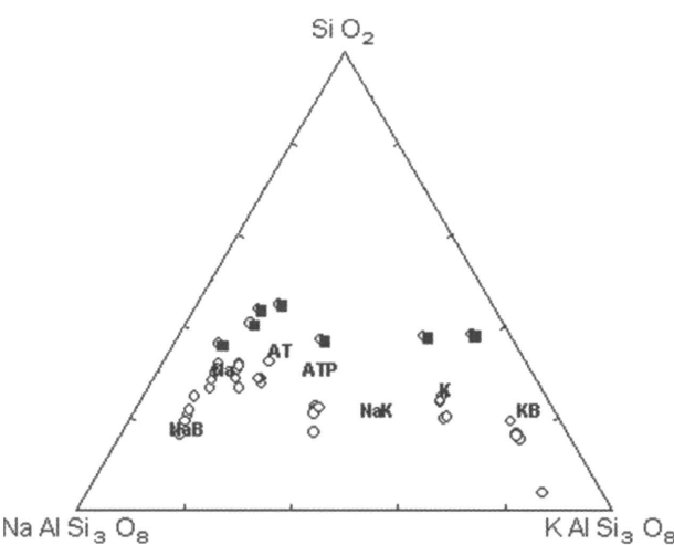
Figure 5. Plot of liquid phase compositions in the ternary diagram \text{SiO}_2\text{-NaAlSi}_3\text{O}_8\text{-KAlSi}_3\text{O}_8 at increasing temperatures (1100-1200°C) for time corresponding to the maximum densification. Black squares = bulk composition of the porcelain stoneware body.
