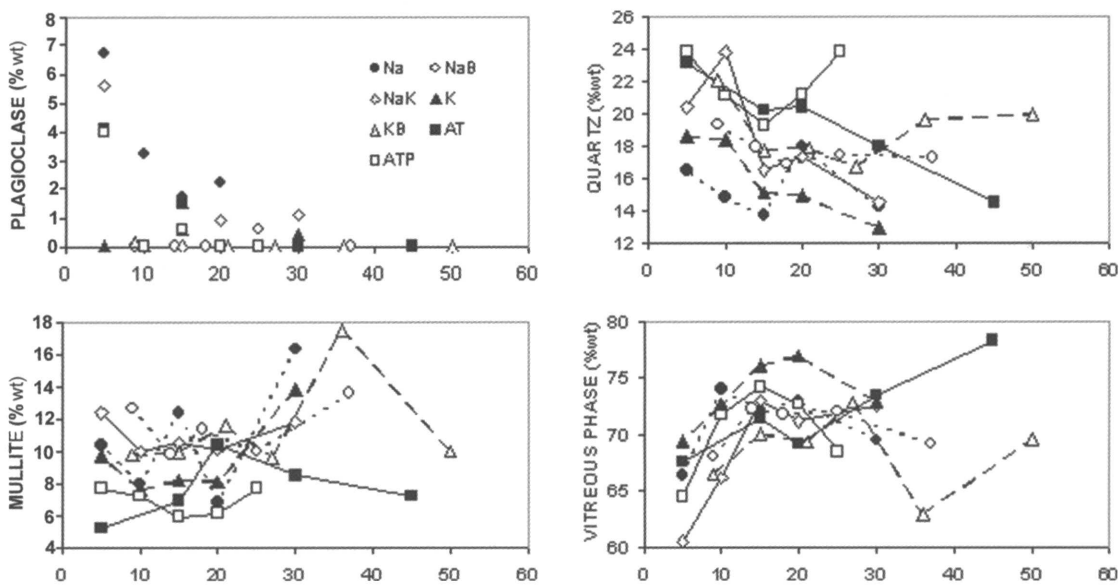
Figure 8. Phase transformations during the isothermal sintering (1200°C) of different porcelain stoneware bodies.
