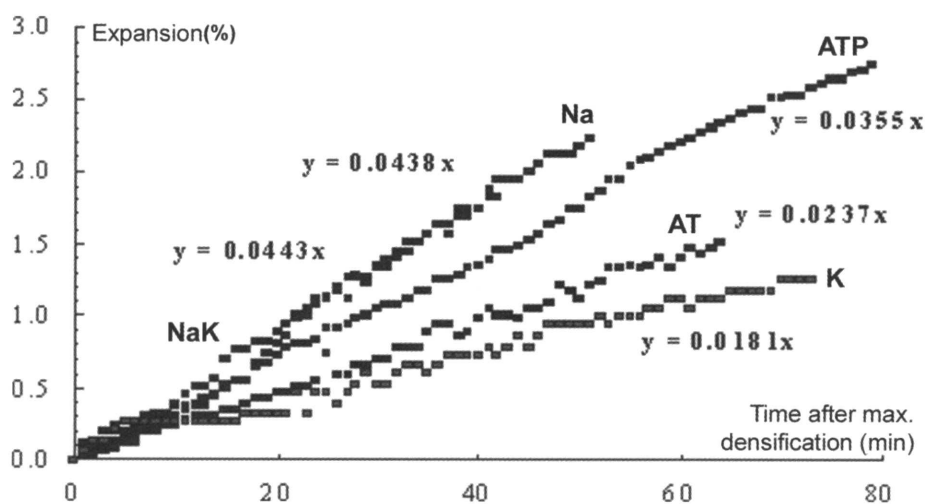
Figure 12: Correlation between the time after maximum densification and the expansion.
