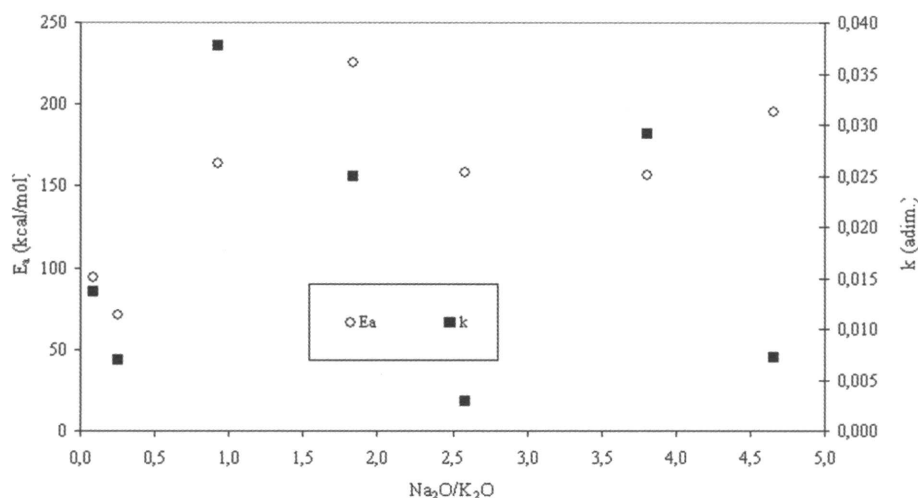
Figure 10: Correlation between the Na/K ratio of porcelain stoneware bodies with the apparent energy of activation of the viscous flow ( E_a ) and the Avrami kinetic parameter k .
