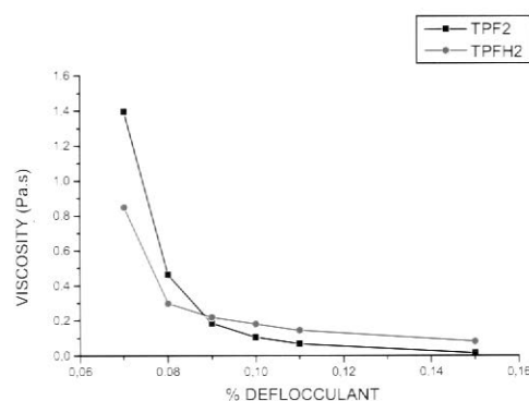
Figure 6 – Evolution of viscosity vs STP2 % in natura and hydrated.
