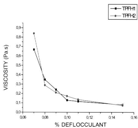
Figure 4 – Evolution of viscosity vs STP% hydrated.
