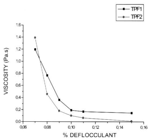
Figure 3 – Evolution of viscosity vs STP% in natura.
