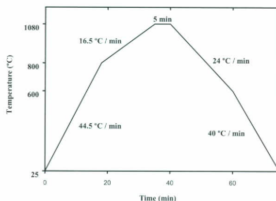
Figure 3. Glaze firing cycle used.
