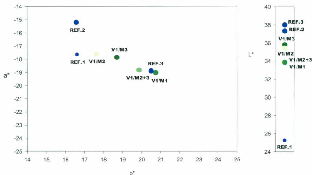
Figure 5. Study of the mineraliser.
