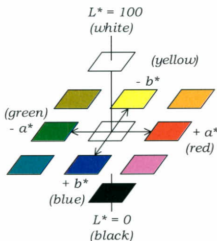
Figure 4. Spatial representation of the values L^* , a^* and b^* .
