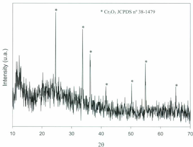
Figure 8. XRD of calcined sample V2/M2/1.
