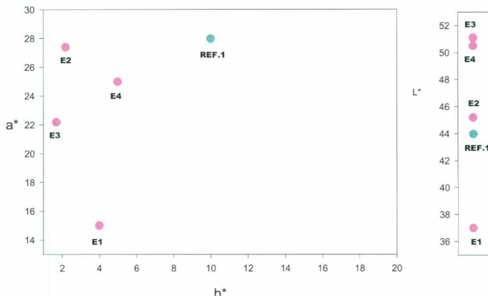
Figure 14. Chromatic co-ordinates of the chromium-tin pigment.
