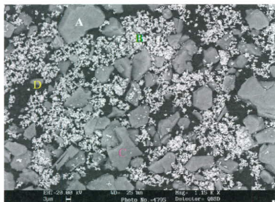
Figure 10. SEM of calcined V2/M2/1 without washing.
