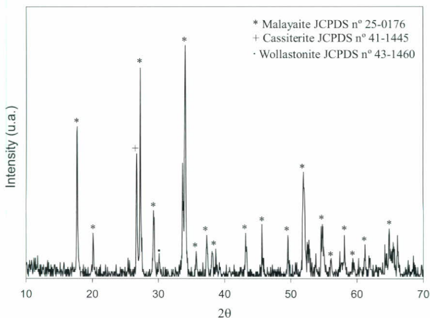
Figure 15. XRD of calcined sample E2.
