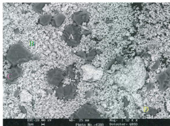
Figure 11. SEM of calcined V2/M2/1 without washing.
