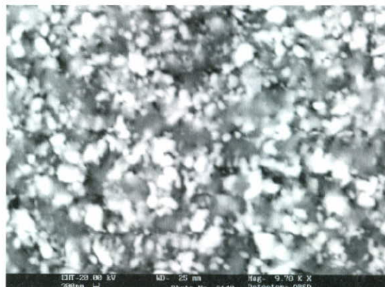
Figure 13. SEM of V2/M2/1 calcined and washed with H 2 O.
