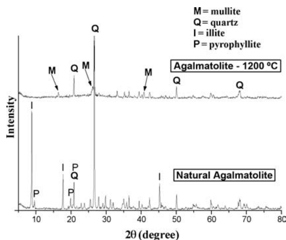
Figure 3. Diffractograms of samples of natural agalmatolite and sintered agalmatolite at a temperature of 1200 °C.
