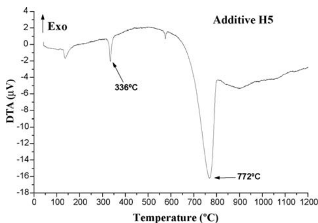
Figure 4. Differential thermal analysis of H5 additive.
