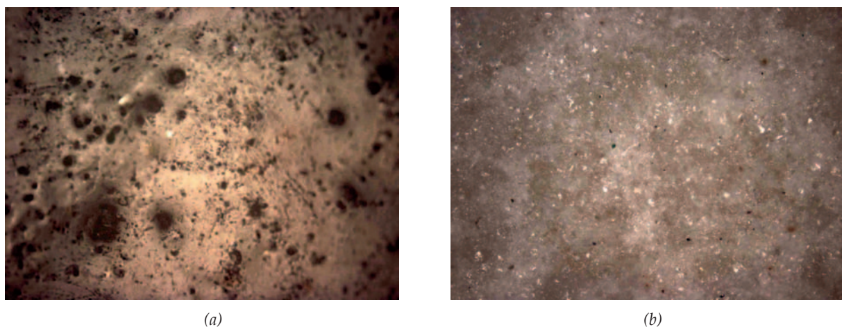
Figure 5. Micrographs obtained in OM of body tests without polishing of the STD piece (a) and H5 (b) with a magnification of 100x.
