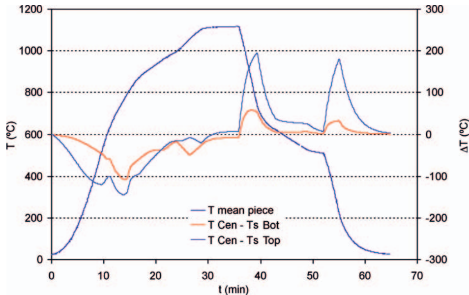
Figure 12. Temperature difference between the tile centre and surface.
