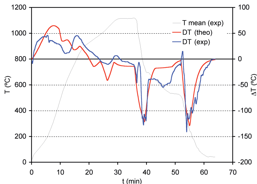
Figure 11. Temperature difference between the top and bottom surfaces ( T_{top} - T_{bot} ) of the tile during industrial firing. Comparison of the theoretical and experimental values.
