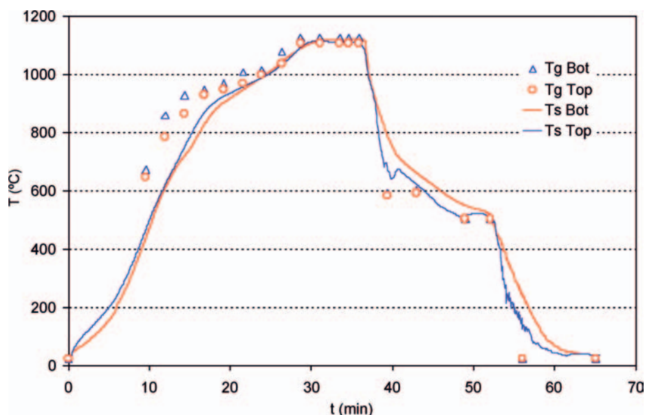
Figure 7. Kiln gas temperature ( T_g : circles (top zone) and triangles (bottom zone)) and tile surface temperature ( T_s : solid lines).
