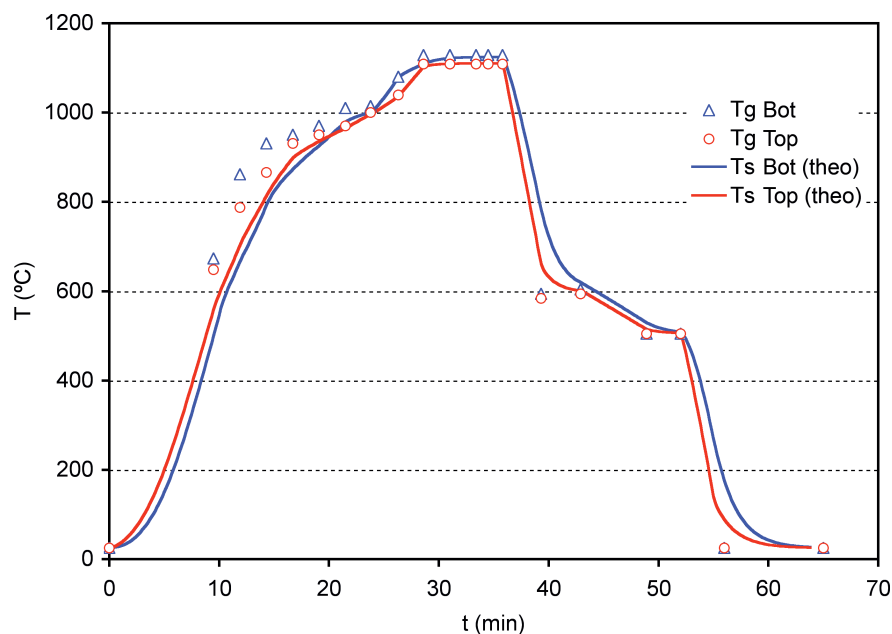
Figure 10. Temperature recorded by the thermocouples (points) and temperature curve of the tile surface calculated from the model developed.
