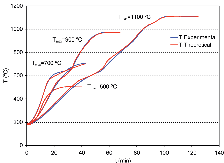
Figure 3. Evolution of temperature in the centre of the tile. Comparison of experimental and theoretical results.
