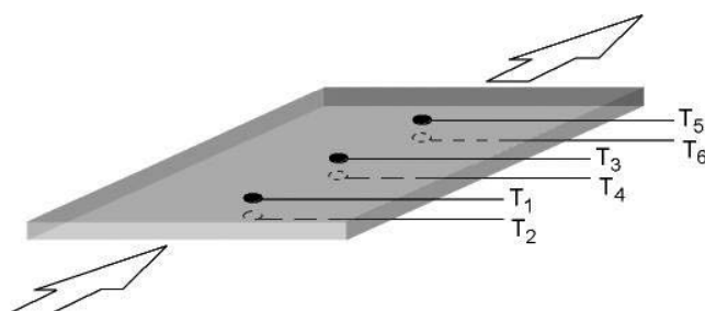
Figure 4. Position of the thermocouples on the tile surface.
