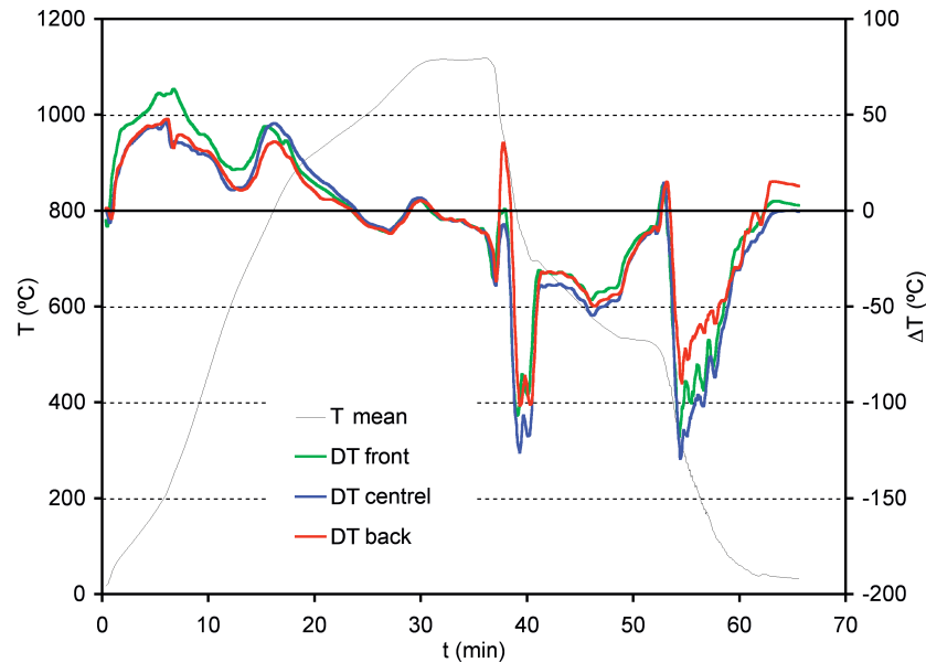
Figure 8. Mean temperature, and difference in temperature between tile top and bottom surfaces in three regions of the tile.
