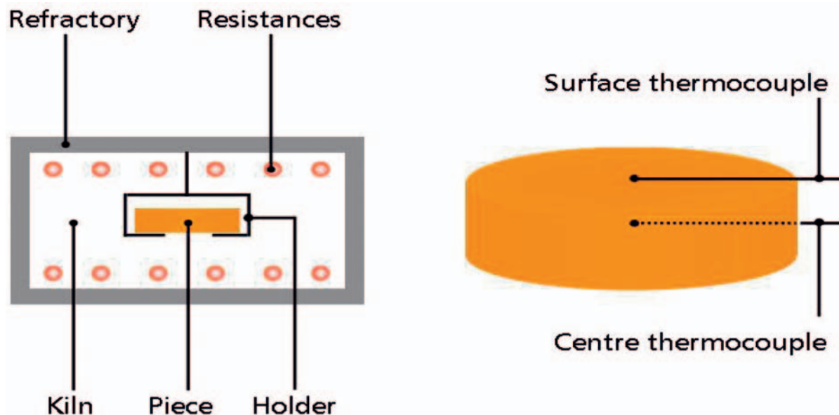
Figure 2. Set-up used to measure the thermal properties.
