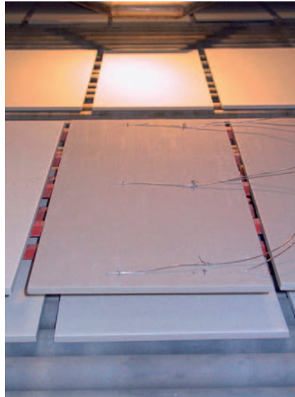
Figure 5. Picture of the tile with the six fitted thermocouples.
