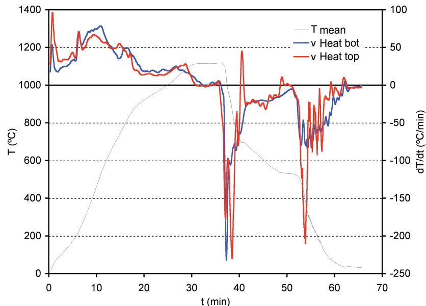
Figure 9. Heating and cooling rates at the tile surfaces.
