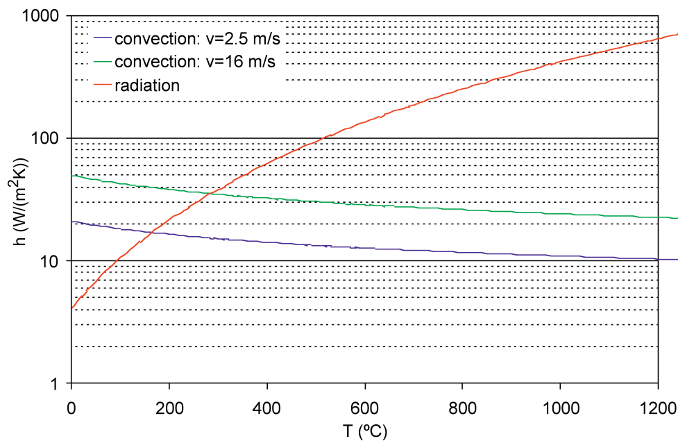
Figure 1. Coefficients of heat transmission by convection and radiation versus temperature.
