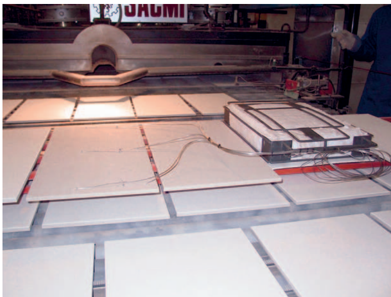
Figure 6. Photograph of the sensorised tile–Datapaq probe assembly before the assembly entered the kiln.
