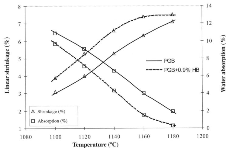
Figure 6. Vitrification diagrams of the white-firing stoneware floor tile compositions.
