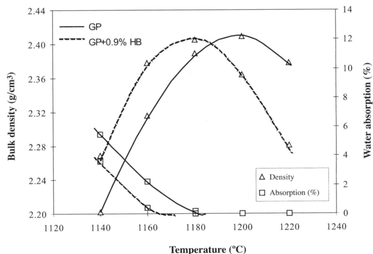
Figure 7. Vitrification diagrams of the porcelain tile compositions.
