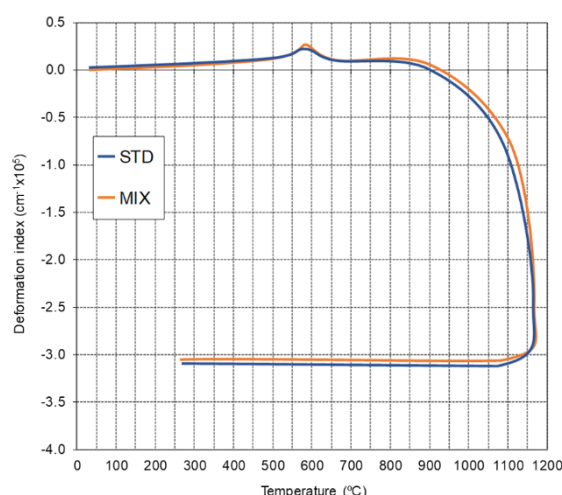
Figure 11. Deformation curves obtained for both materials.
