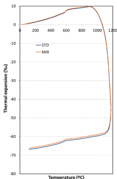
Figure 9. Expansion-shrinkage curves for both tested materials.
