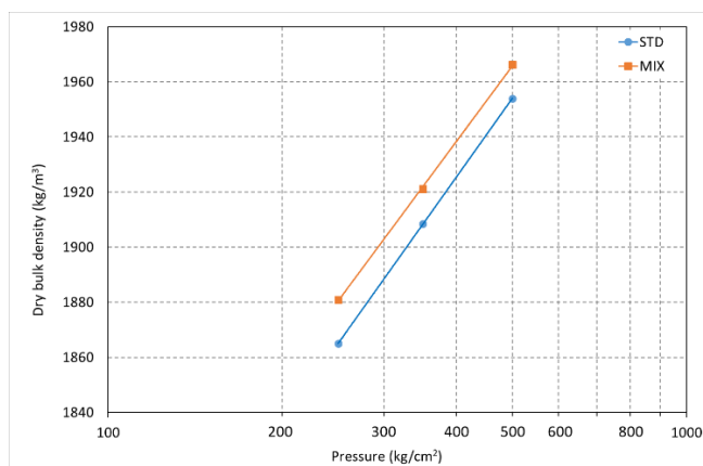
Figure 7. Evolution of dry bulk density with pressing pressure.
