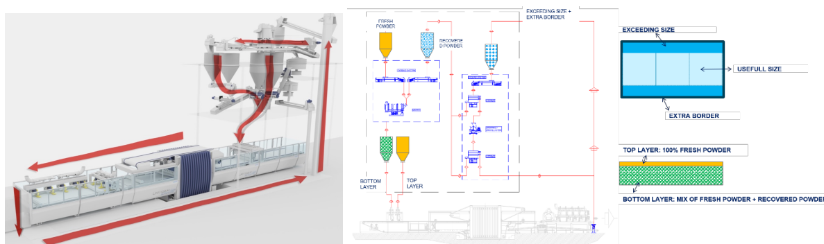
Figure 2. General powder flows in the developed scrap recovering system (left) and detail of the different powder layers constituting the product (right).
