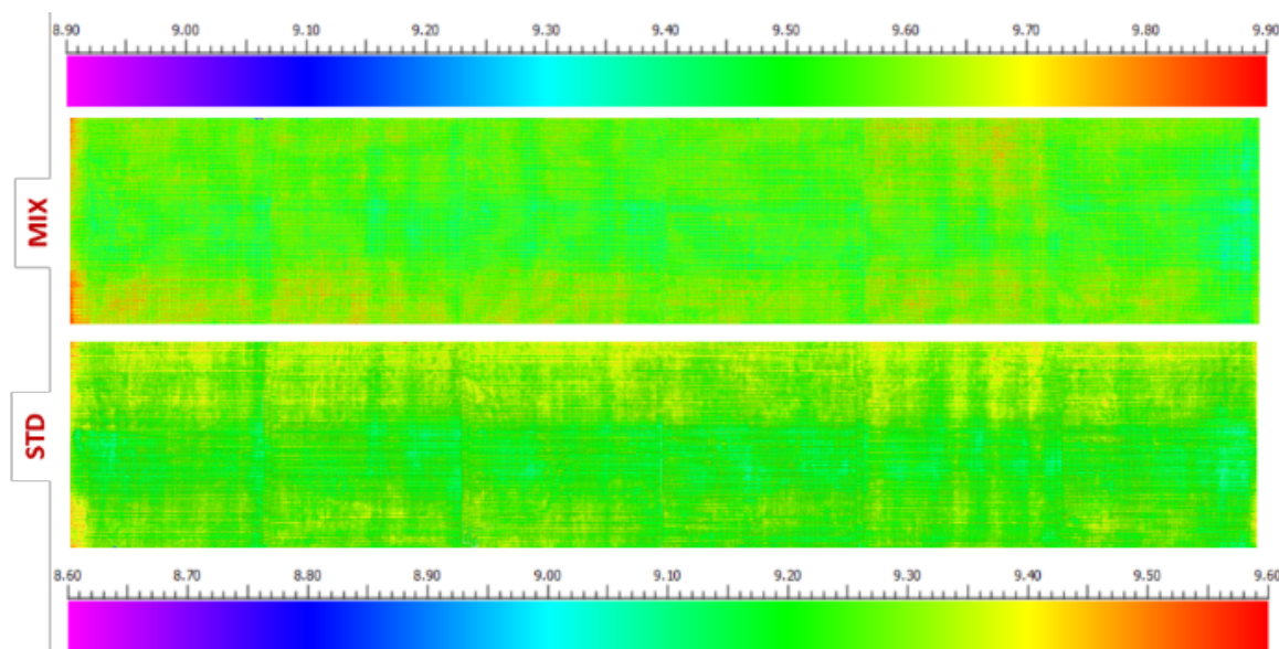
Figure 13. Thickness (mm) distribution of six fired 900 mm x 900 mm tiles obtained from green cutting of a big slab.
