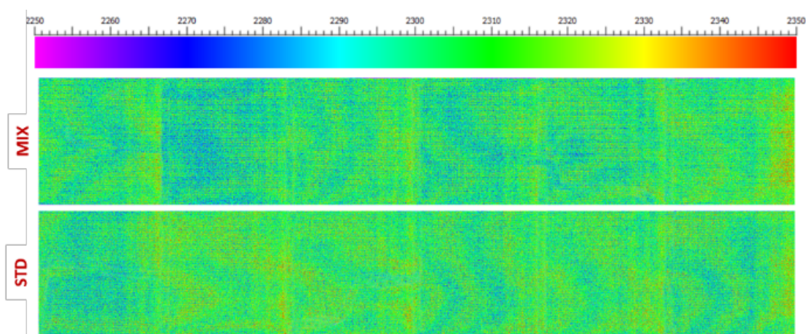
Figure 12. Fired density (kg/m 3 ) distribution of six 900 mm x 900 mm tiles obtained from green cutting of a big slab.
