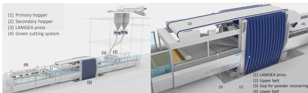
Figure 1. LAMGEA® shaping line (left) and details of the LAMGEA® press and conveying system (right).
