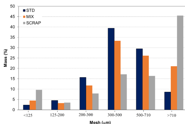
Figure 3. Granule size distribution.
