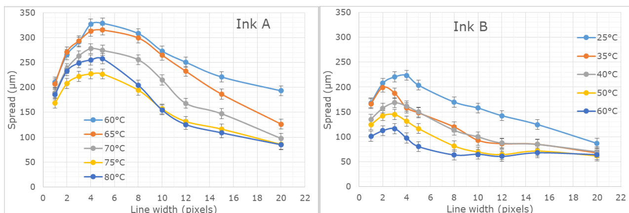
Fig.9: Measure of spread for ink A and B at various glass temperatures and increasing line width.
