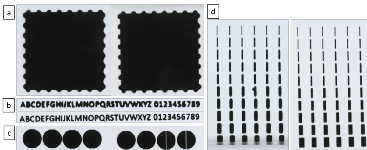
Fig.8: Image printed on a glass with ink B, taken with a high-resolution scanner (1200 dpi): on the left 25°C, on the right 40°C glass temperature. Letters printed at 25°C are the upper ones. Description as in Fig.7.
