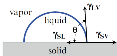
Fig.1: Schematic representation of a drop on a solid surface, with indication of the solid, liquid and solid-liquid surface tensions and contact angle \theta .
