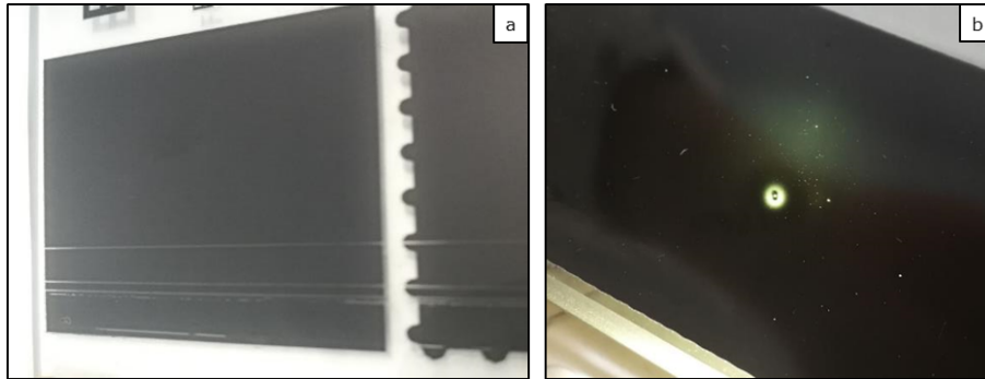
Fig.6: a) Missing nozzle defect and b) a "hole" defect in a full shade printed on glass.
