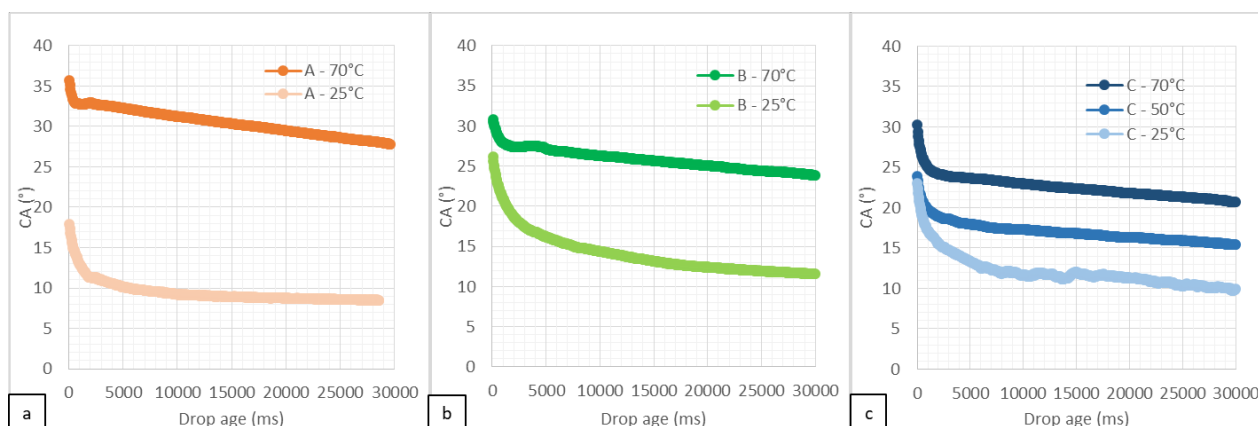
Fig.4: Contact angle measurements for three different ink samples at various substrate temperatures as a function of drop age: a) ink A with substrate at 25 and 70°C, b) ink B with substrate at 25 and 70°C, c) ink C with substrate at 25, 50 and 70°C.
