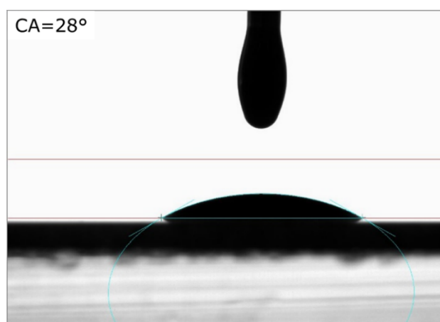
Fig.3: Example of contact angle images taken with OCA100 for ink on glass. The operator positions the red as a reference for air and base line. Blue lines indicate the fitting results.
