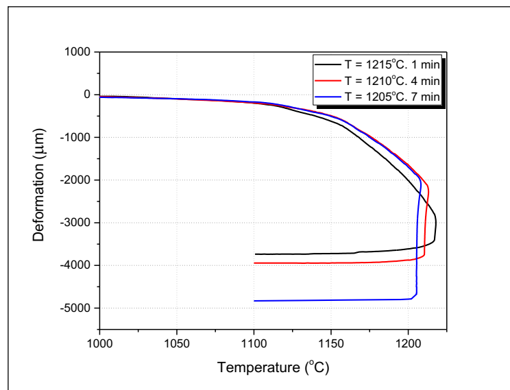
Fig.2 Deformation of the samples during firing at different thermal cycles.
