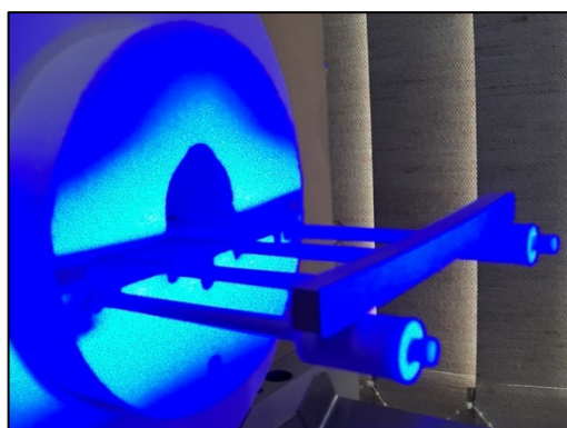
Fig.1 Experimental setup used to evaluate the pyroplastic deformations of the samples.
