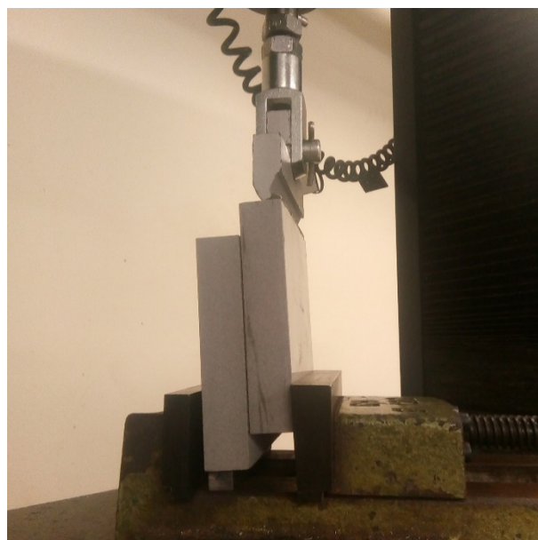
Figure 1. Assembled two-tile test specimen in the shear test stand of the universal testing machine.
