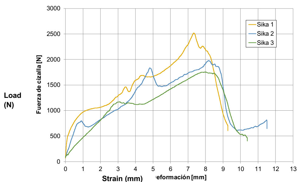
Figure 2. Load-strain curves of the Sikaflex 265 adhesive after 7 days maturing.
