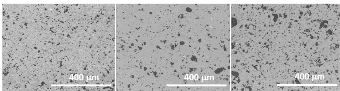
Figure 2. Microstructure of fired body specimens sintered at the maximum densification temperature obtained from 1-STD, 3-STD and 6-STD compositions (from left to right).
