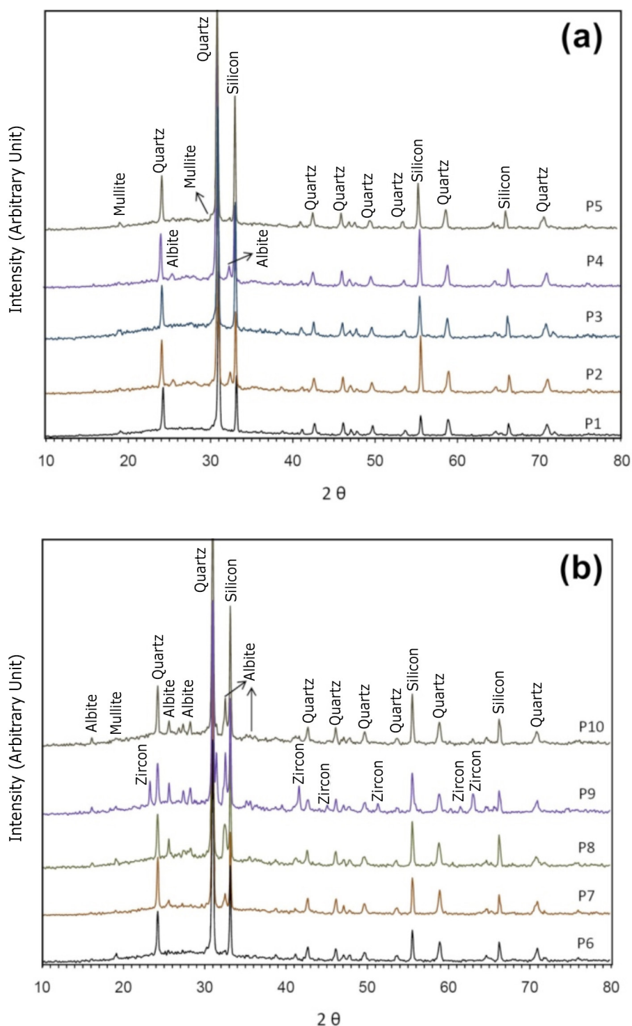
Fig. 3. XRD analysis of samples: (a) Samples P1-P5 and (b) samples P6-P10.
