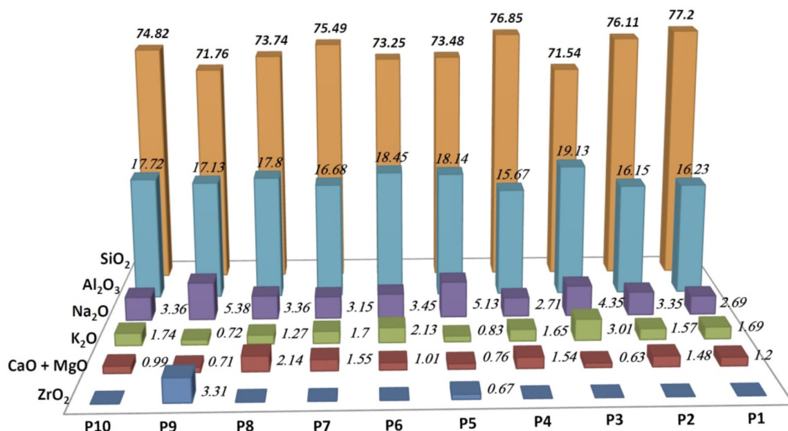
Fig. 2. Chemical analysis (wt.%) of the samples ( \text{Fe}_2\text{O}_3 + \text{TiO}_2 < 1.4\% for all samples).
