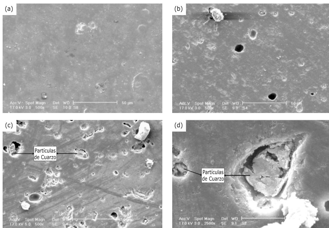
Fig. 5. SEM micrograph of samples (a) P1, (b) P5 and (C & d) P8 (Mag. \times 500 for a, b and c & Mag. \times 2500 for d).
