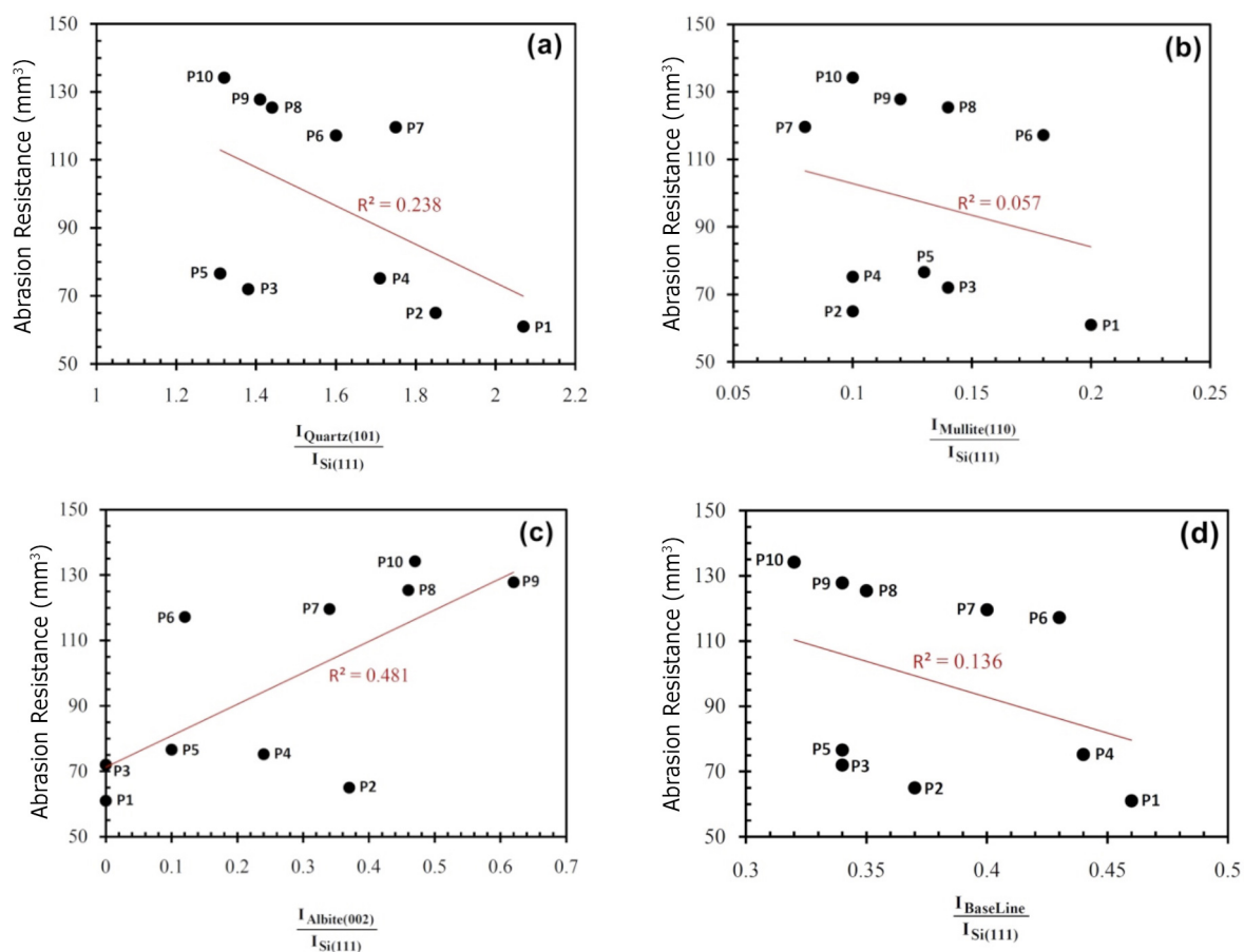
Fig. 4. Correlation between abrasion resistance and the amount of identified phases. Abrasion resistance versus (a) Quartz, (b) Mullite, (c) Albite and (d) amorphous phase.
