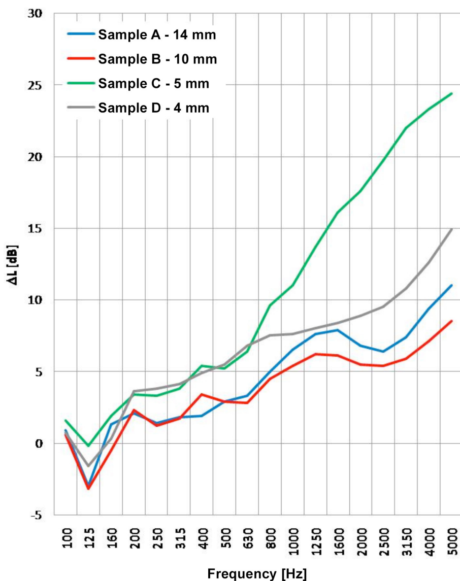
Figure 3: Noise changes as a function of frequency for all the samples having different thickness.
