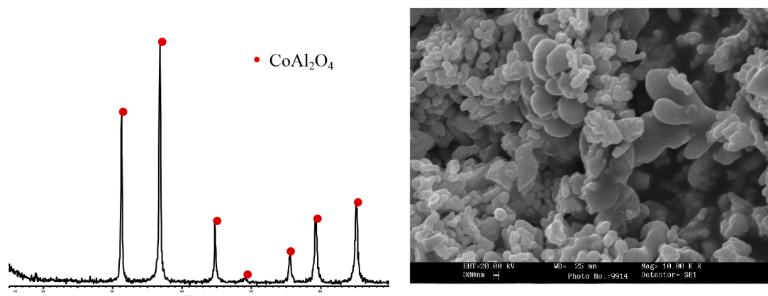
Figure 2. Diffraction pattern and micrograph of a pigment sintered in situ by laser technology.
