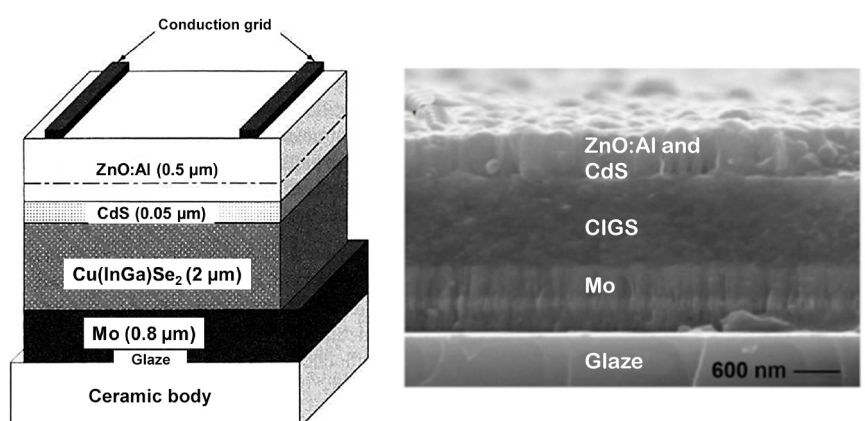
Figure 4. Photovoltaic solar cell of chalcopyrite (CIGS) and its corresponding cross-sectional SEM micrograph.
