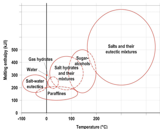
Figure 3. Melting enthalpy as a function of the temperature range, different groups of phase change materials (PCM). Ref. "J. Dieckmann, Latent heat storage in concrete."
