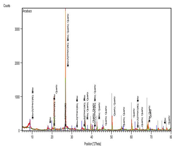
Figura 13. Diffractograma material Arcabuco
