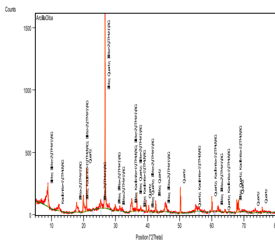
Figura 10. Difractograma Cumbre-Santander
