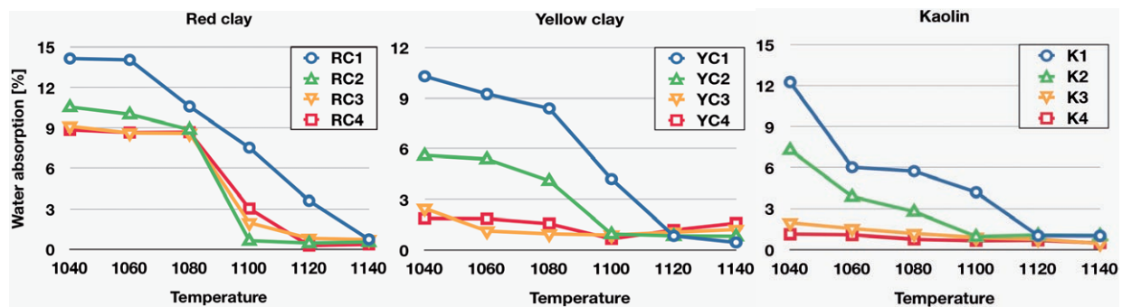
Figure 2. Water absorption of the samples prepared.
