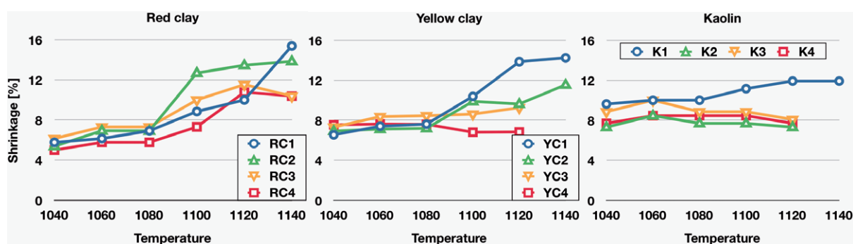
Figure 1. Shrinkage of the samples prepared.
