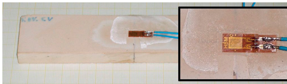
Figure 8. Residual stress measurement test and detail of the gauge.
