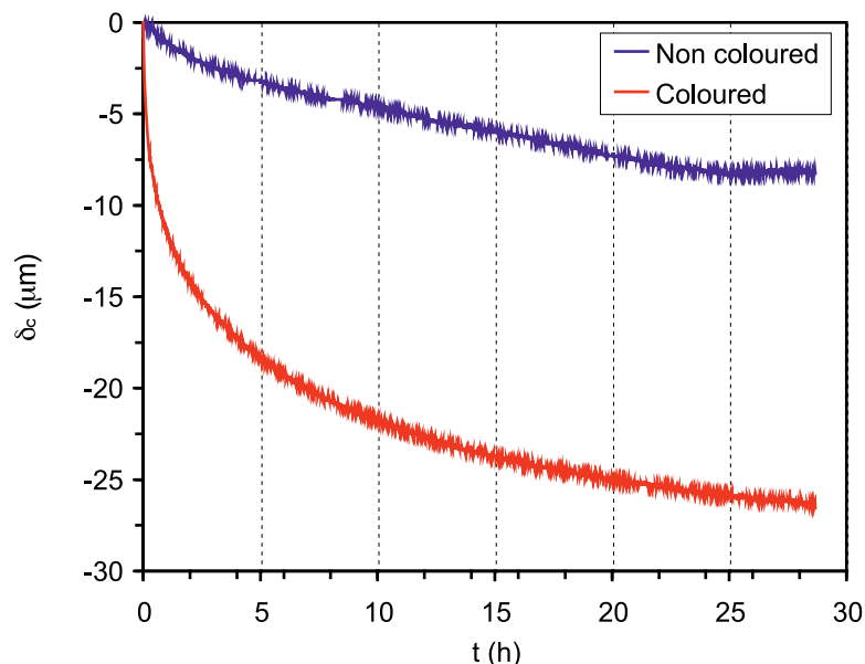
Figure 18. Influence of dry colouring on creep.
