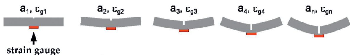
Figure 9. Schematic illustration of the principle of the method used to measure the residual stresses.
