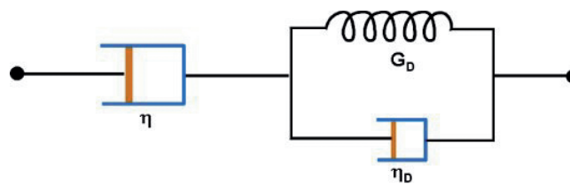
Figure 15. Linear viscoelastic model used to model creep.
