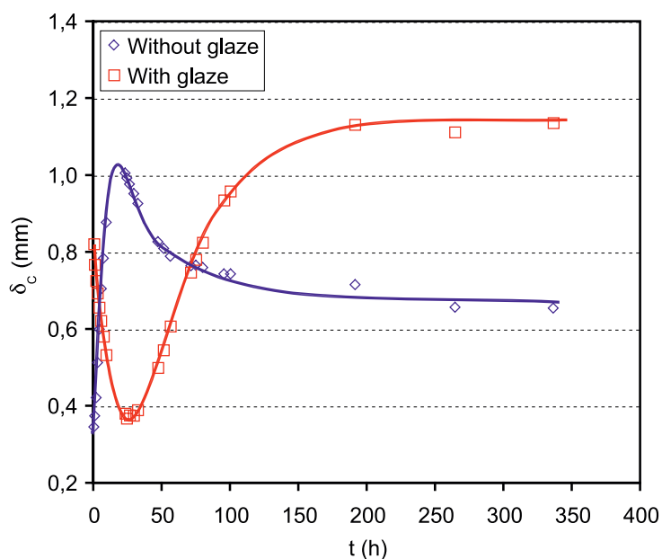
Figure 19. Evolution of tile deflection with and without glaze.
