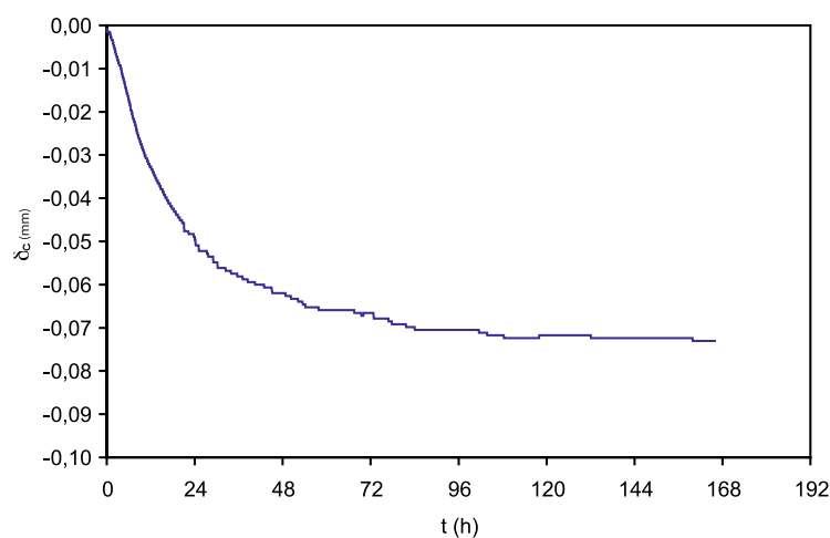
Figure 7. Delayed curvature caused by expansion of the body.
