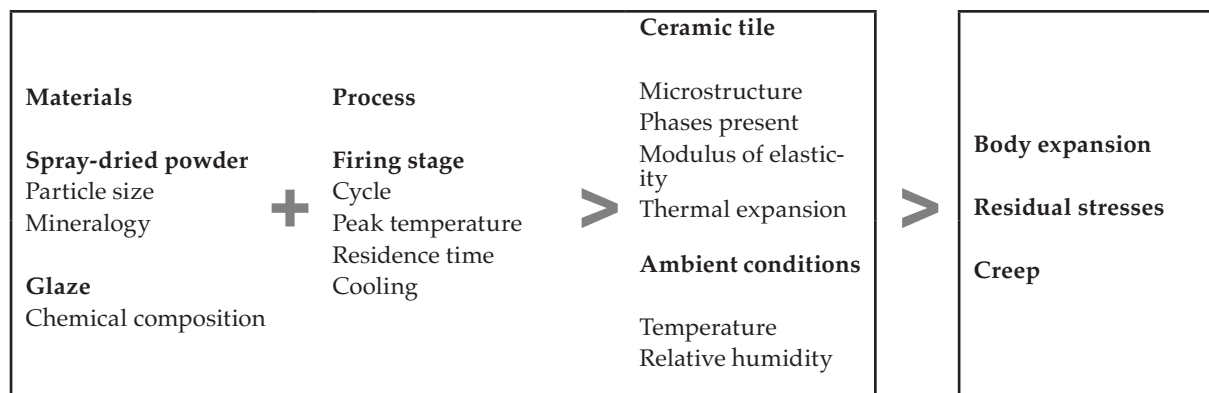
Figure 16. Factors that influence delayed curvatures
