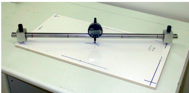
Figure 1. Arrangement used to measure the deflection of industrial tiles.
