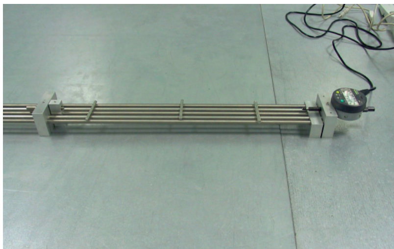
Figure 5. Device that automatically offsets temperature for the measurement of body expansion.
