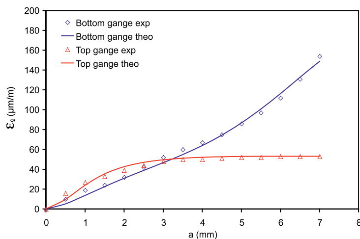
Figure 11. Experimental strain and fit for a porcelain tile.
