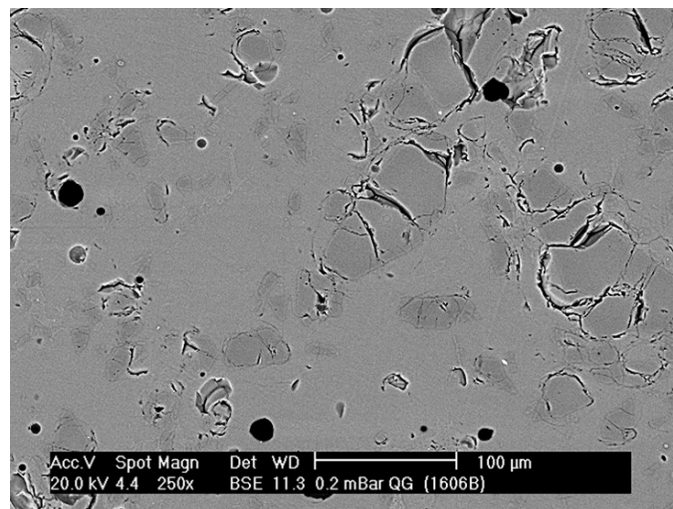
Figure 17. Cross-section of a porcelain tile.
