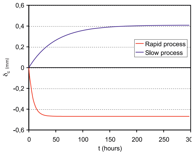
Figure 3. Contribution of both processes. Model-1, Tile 2.
