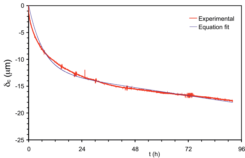
Figure 14. Strain of a porcelain tile test piece under loading.
