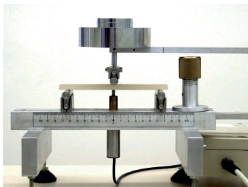
Figure 13. Device used to measure creep.
