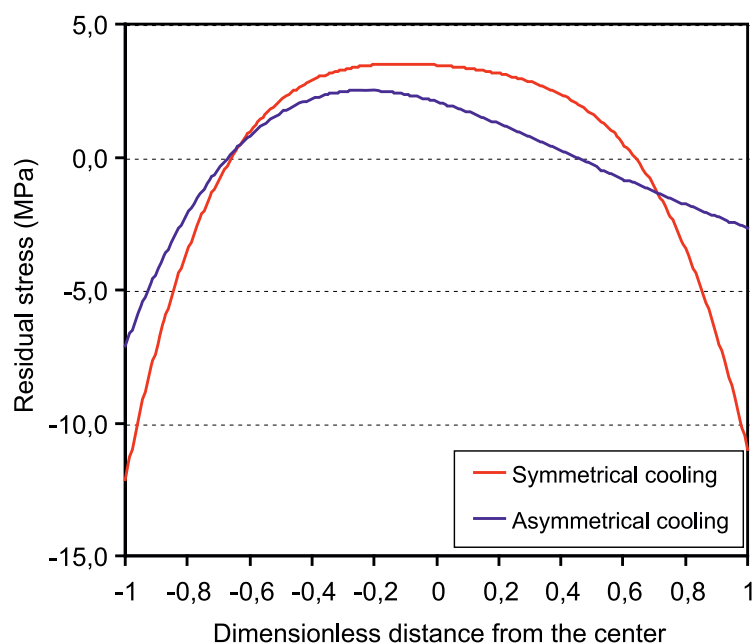
Figure 20. Residual stress profile as a function of type of cooling.
