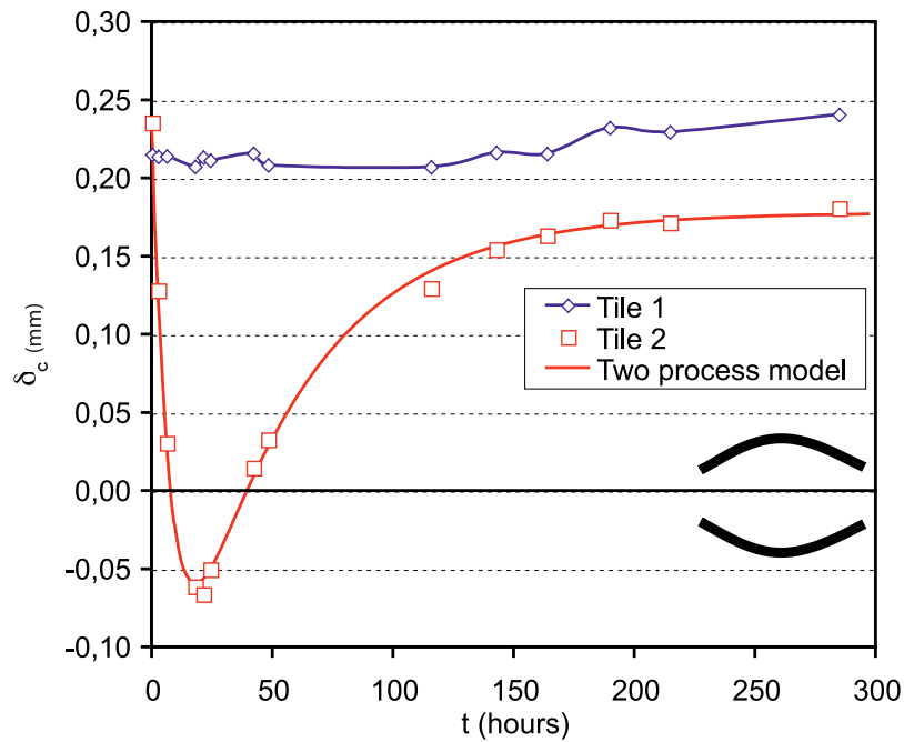
Figure 2. Evolution of deflection in industrial tiles. Model 1.
