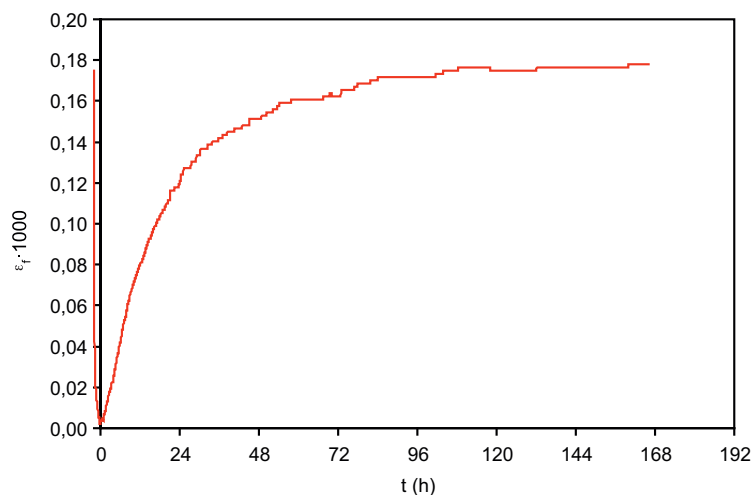
Figure 6. Evolution of the expansion of a porcelain tile body as a function of time.
