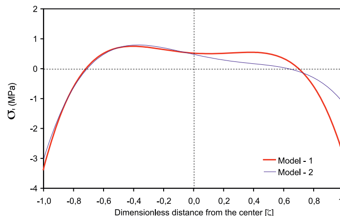
Figure 12. Residual stress profiles of Model-1 and Model-2.
