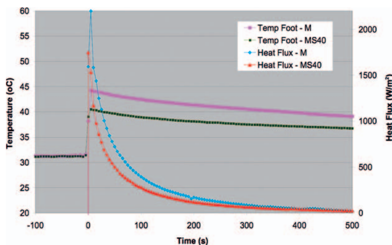
Figure 10. Relationship between temperature and time during barefoot-flooring contact.
