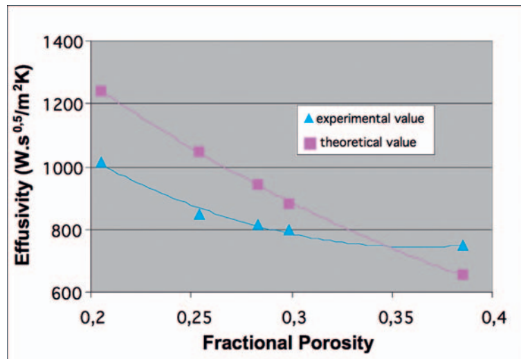
Figure 9. Measured and theoretical thermal effusivities as a function of porosity (silica fibre contents ranging from 0 to 40wt%) for samples compacted at 30 MPa.
