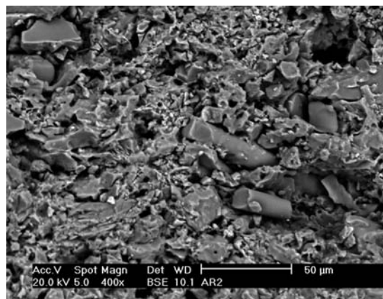
Figure 5. SEM micrograph related to a ceramic sample with 10 wt% amorphous silica fibres incorporated. Magnification: 400 X.
