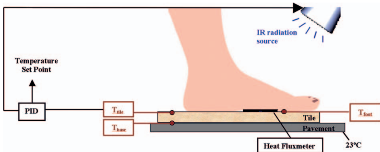
Figure 1. Schematic illustration of the experimental apparatus used in this work.
