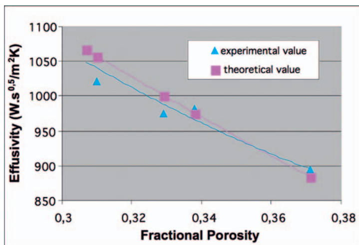
Figure 7. Measured and theoretical thermal effusivities as a function of porosity (compaction pressure ranging from 30 to 10 MPa) for samples without silica fibres.
