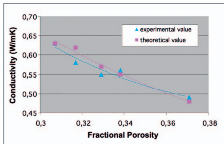
Figure 6. Measured and theoretical thermal conductivities as a function of porosity (compaction pressure ranging from 30 to 10 MPa) for samples without silica fibres.
