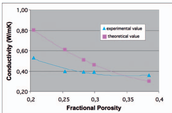
Figure 8. Measured and theoretical thermal conductivities as a function of porosity (silica fibre contents ranging from 0 to 40wt%) for samples compacted at 30 MPa.
