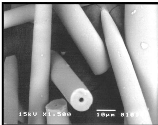
Figure 3. SEM micrograph related to amorphous silica fibres. Magnification: 1500 X
