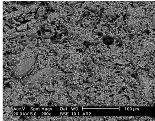
Figure 4. SEM micrograph related to a ceramic sample with 10 wt% amorphous silica fibres incorporated. Magnification: 200 X.
