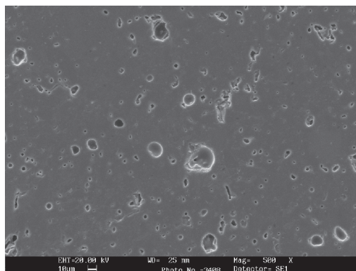
Figure 13. Micrograph (SEM/EDX) of the polished surface of sample P4 fired at 1190.
