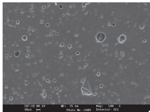
Figure 12. Micrograph (SEM/EDX) of the polished surface of sample P3 fired at 1190 °C.
