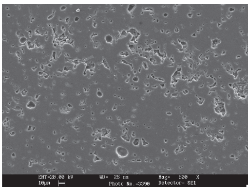
Figure 11. Micrograph (SEM/EDX) of the polished surface of sample P2 fired at 1190 °C.
