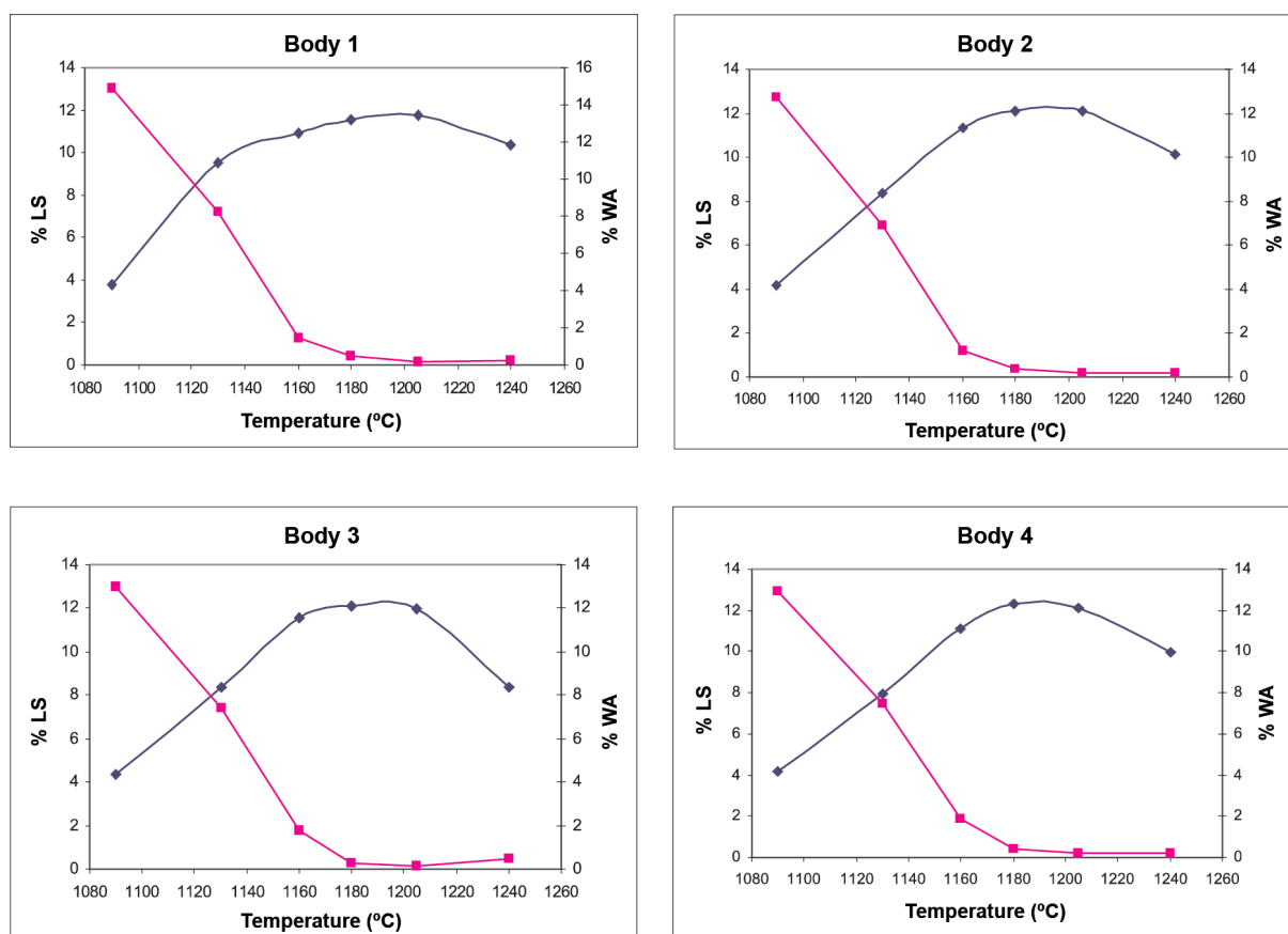
Figures 5-8. Vitrification diagrams of the porcelain tile compositions formed by pressing.
