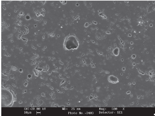
Figure 9. Micrograph (SEM/EDX) of the polished surface of sample P0 fired at 1190 °C.
