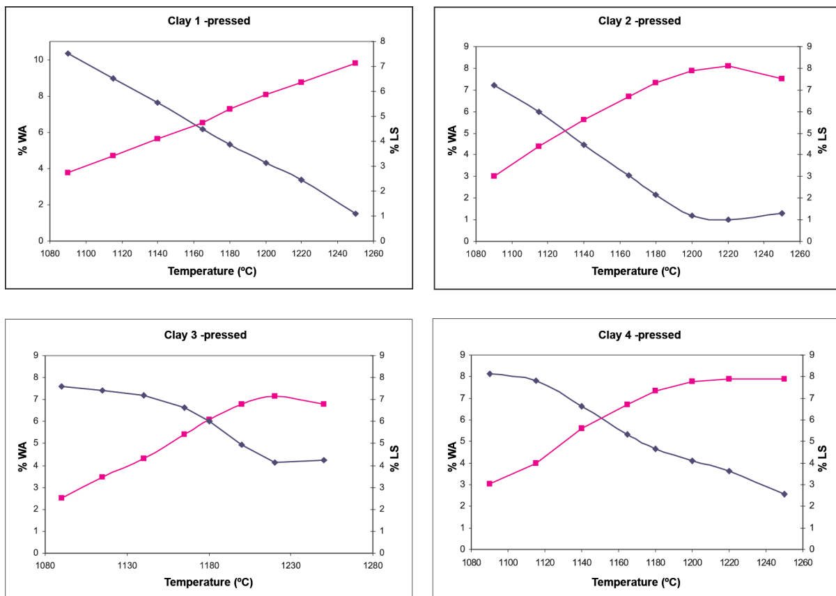
Figures 1-4. Vitrification diagrams of the clays formed by pressing.
