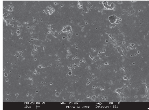
Figure 10. Micrograph (SEM/EDX) of the polished surface of sample P1 fired at 1190 °C.
