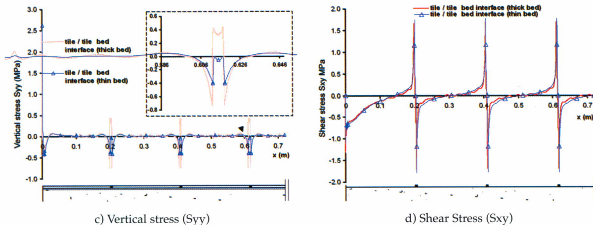
Figure 7 – Thick bed reference model results compared with the thin bed reference model results
