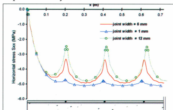
b) Joint width variation
