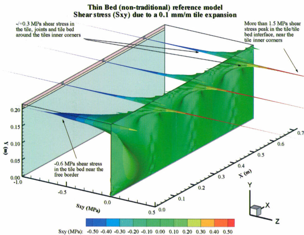
Figure 6 –Thin bed reference model, shear stress ( S_{xy} ) due to a 0.1 mm/m tile expansion
