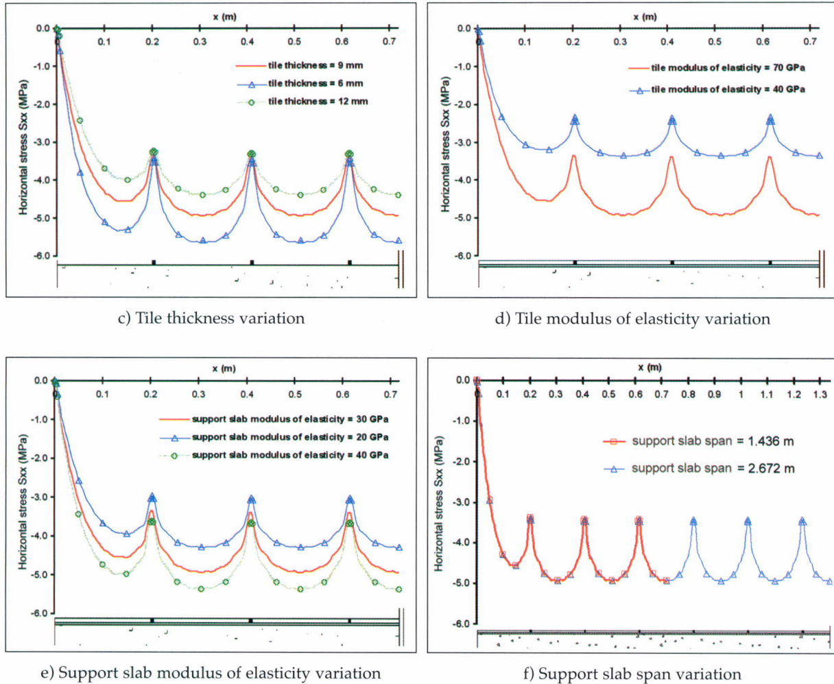
Figure 8 – Parametric study thin bed (non-traditional) model examples, horizontal stress ( S_{xx} ) due to a 0.1 mm/m tile expansion, along the tile cross section
