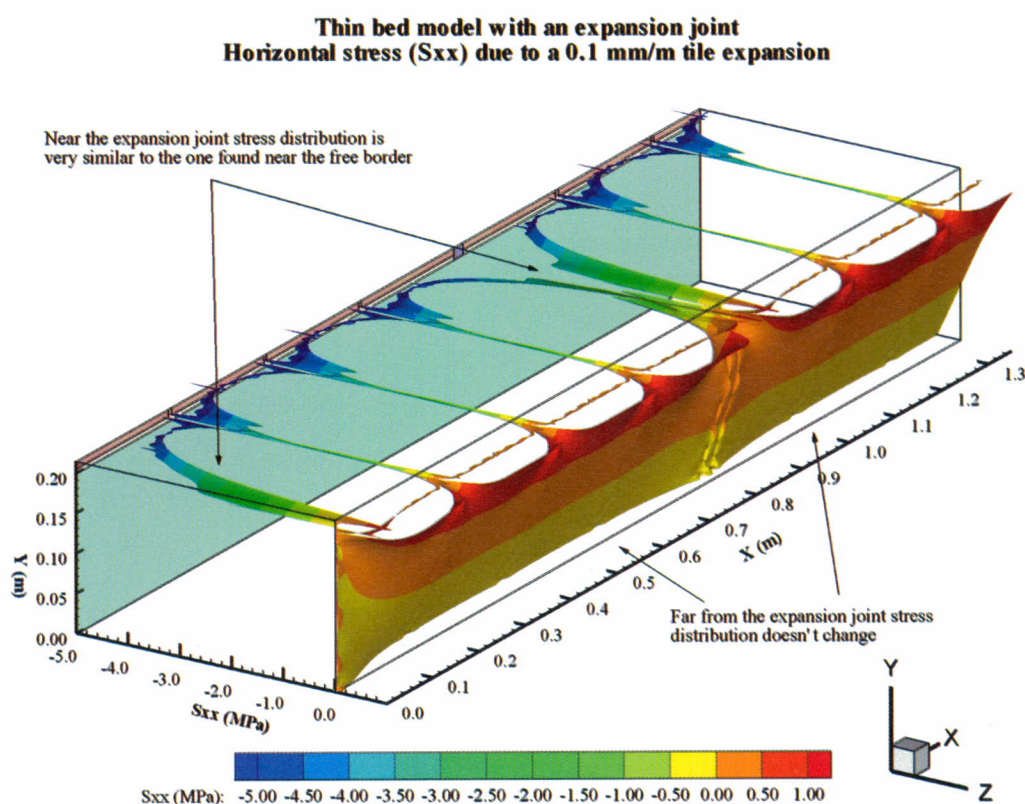
Figure 9 – Thin bed model with an intermediate expansion joint, horizontal stress ( S_{xx} ) due to a 0.1 mm/m tile expansion
