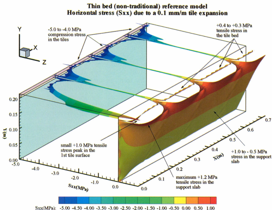
Figure 4 – Thin bed reference model, horizontal stress ( S_{xx} ) due to a 0.1 mm/m tile expansion
