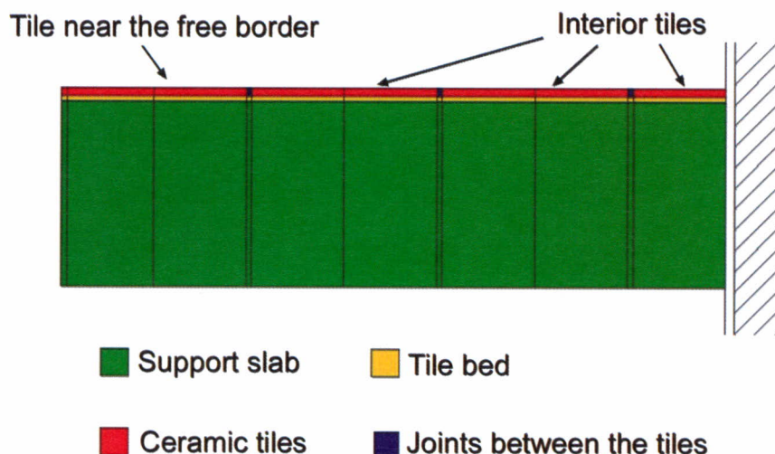
Figure 2 – Thin set reference model: finite element mesh and modelled materials
