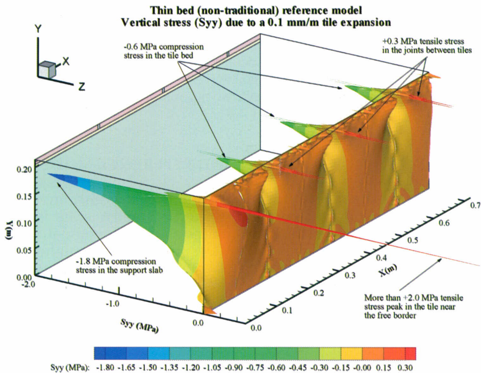
Figure 5 – Thin bed reference model, vertical stress ( S_{yy} ) due to a 0.1 mm/m tile expansion
