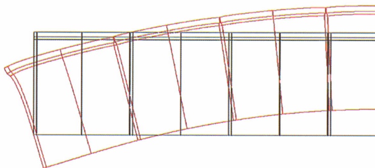
Figure 3 – Model deformed shape (amplified 2300x) due to a 0.1 mm/m tile expansion
