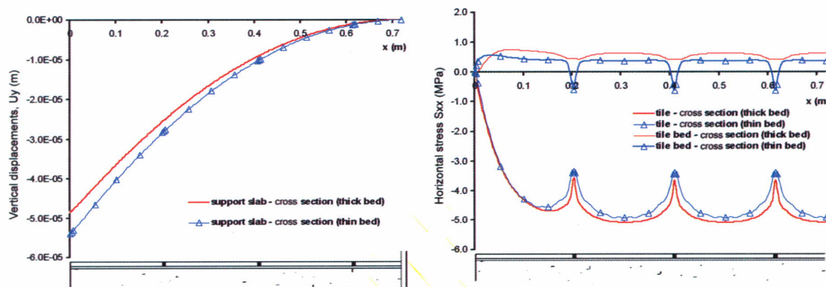
a) Vertical displacements
