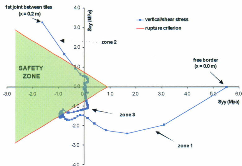
Figure 11 – Shear and vertical stress along the first tile/tile bed interface due to a load combination example compared with a failure condition
