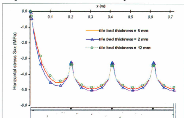
a) Tile bed thickness variation
