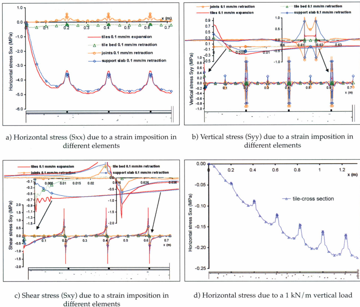
Figure 10 – Stress fields due to various actions, thin bed (non-traditional) reference model
