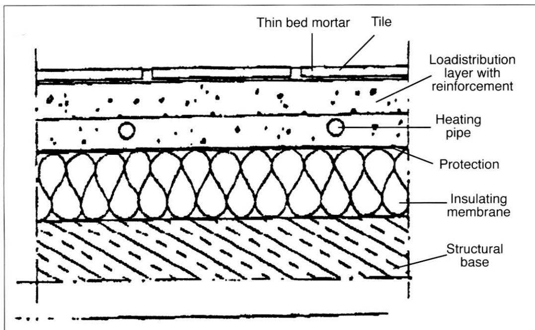
Fig. 3. Thin bed tile installation on a hardened load distribution layer.
