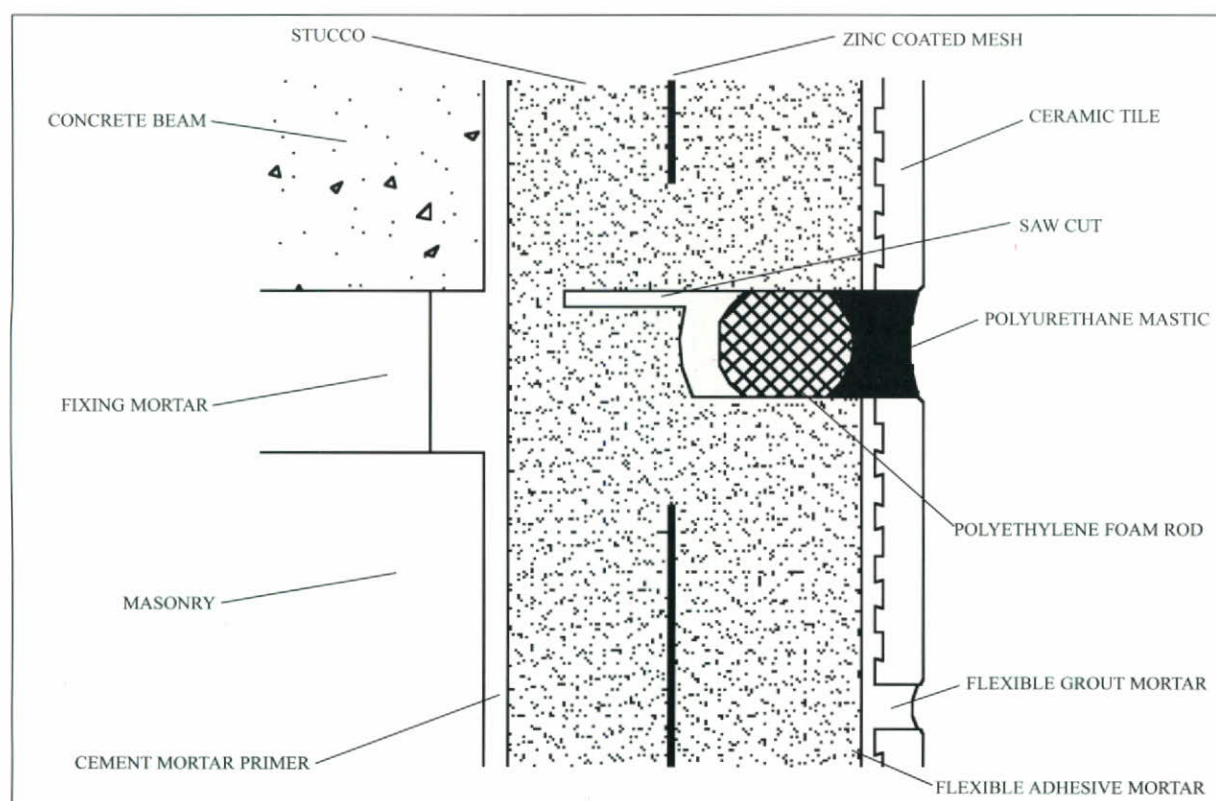
Figure 3. Detail of horizontal control joint for an extruded stoneware tile façade.
