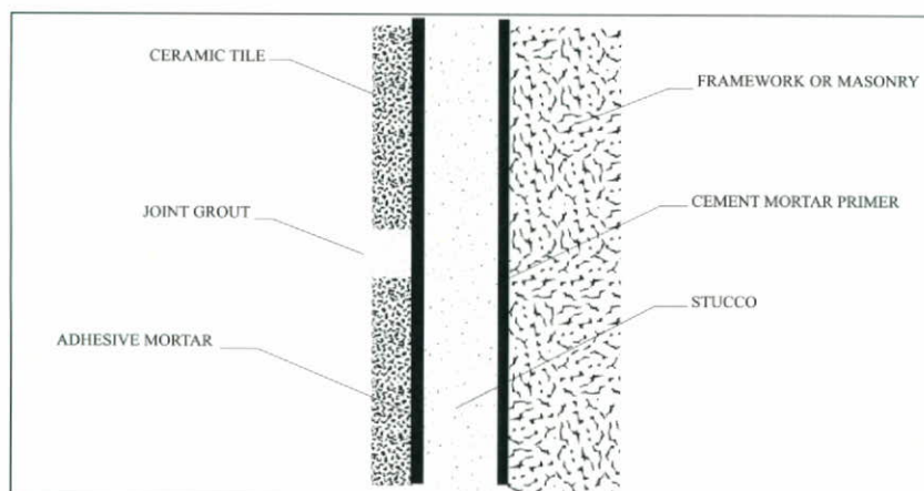
Figure 1. Elements and layers of an adhered ceramic tile façade.
