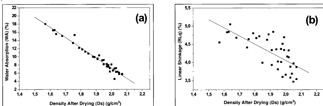
Figure 2: Variation of AA (a) and RLq (b) with the dried density.
