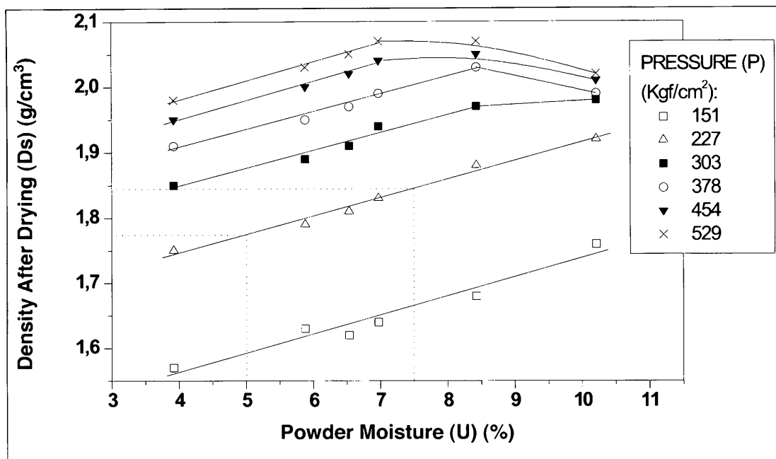
Figure 1: Variation of the dried density ( D_s ) with the moisture of the powder and the compaction pressure.
