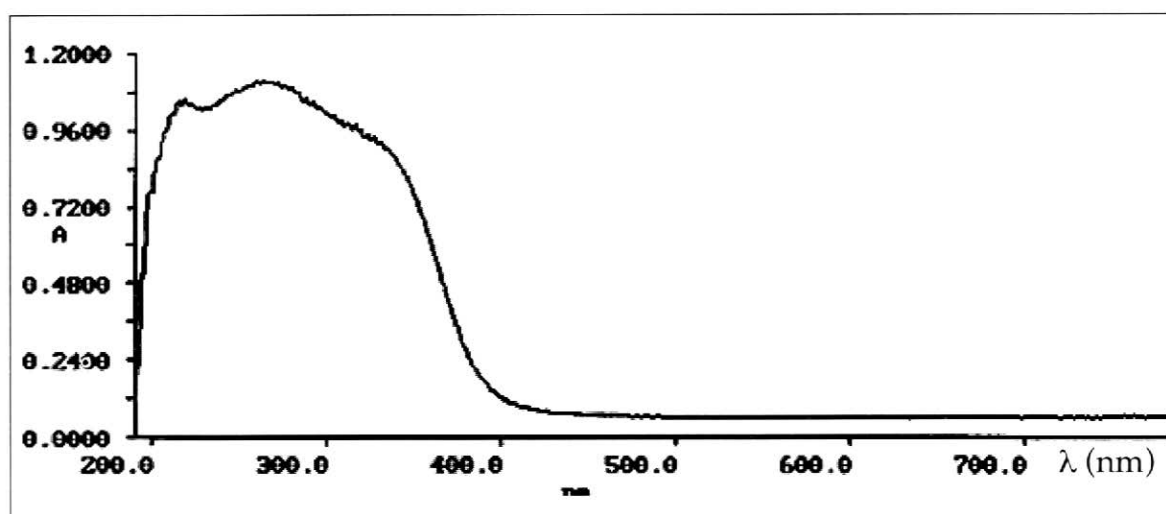
Figure 7. Bactericidal glaze absorption spectrum.
