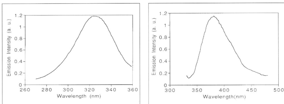
Figure 9. Excitation (A) and emission (B) spectra of the developed material.
