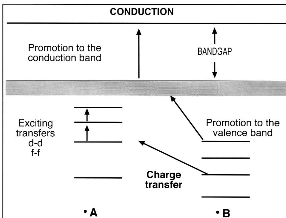
Figure 1. Electron transfers in solids affecting optical properties. Energy levels are shown for two atoms, A and B, together with some characteristic electronic states in solids.
