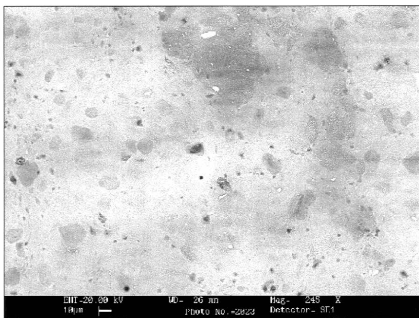
Figure 3. SEM micrograph obtained by secondary electrons.
