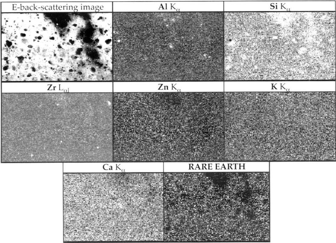
Figure 5. Elemental surface distribution analysis by mapping.
