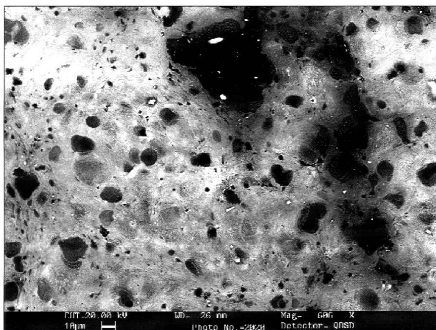
Figure 4. SEM micrograph obtained by back-scattered electrons.
