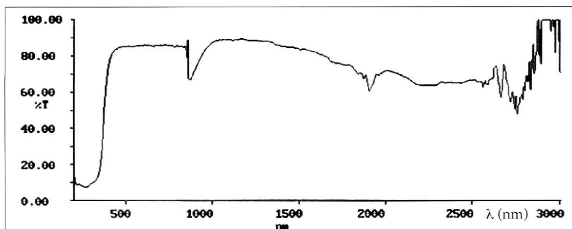
Figure 8. Bactericidal glaze transmittance spectra.
