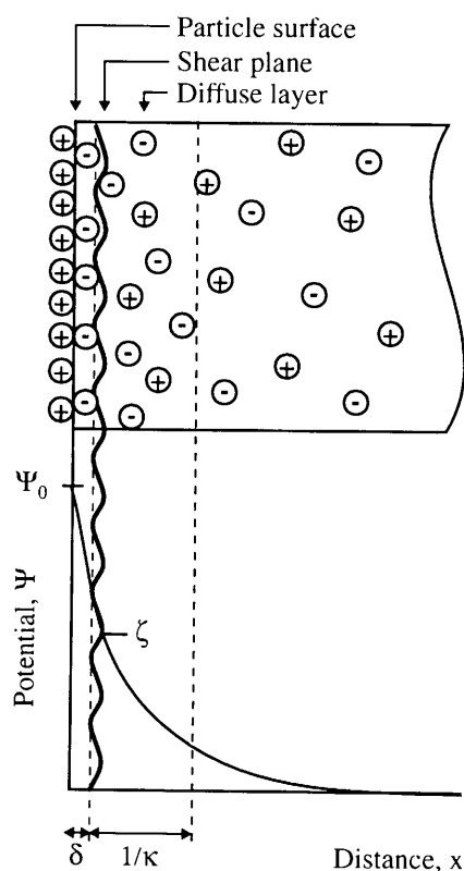
Figure 2. Structure of the electric double layer according to the Stern model.
