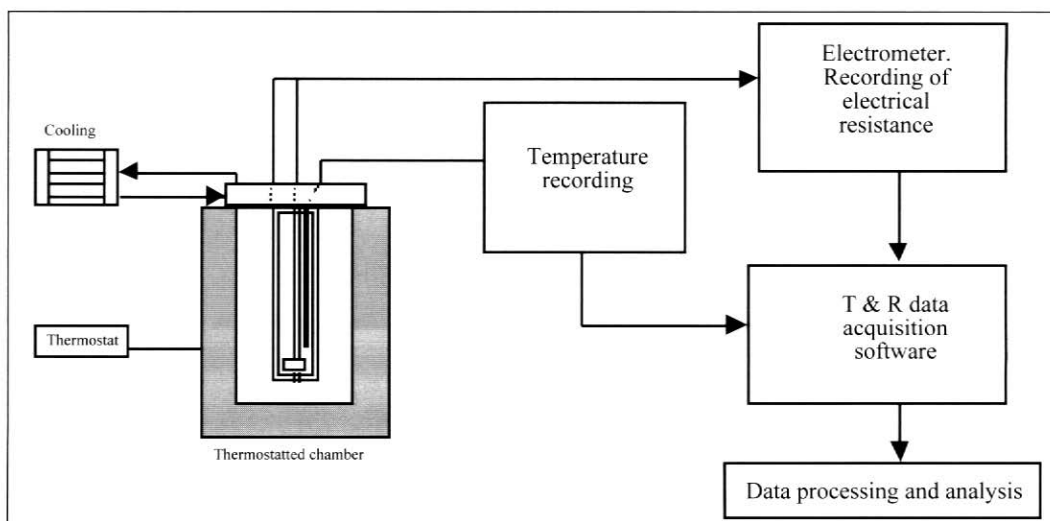
Figure 3. Experimental electrical measuring assembly.
