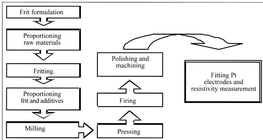
Figure 2. Experimental scheme followed in specimen preparation up to measurement.
