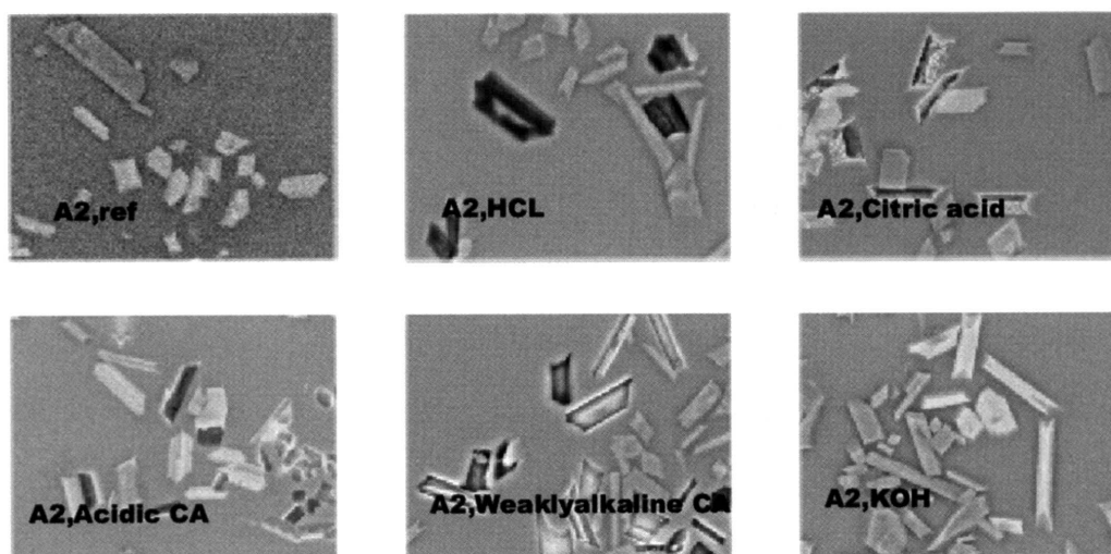
Figure 2. SEM-images of the surface of Glaze A2 before and after exposures to different test solutions. CA=cleaning agent
