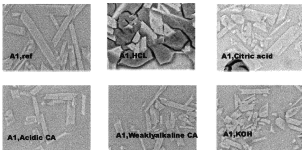
Figure 1. SEM-images of the surface of Glaze A1 before and after exposure to different test solutions as specified in the images. CA=cleaning agent
