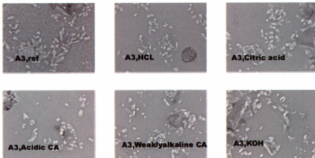
Figure 3. SEM-images of Glaze A3 before and after exposures to different test solutions. CA=cleaning agent
