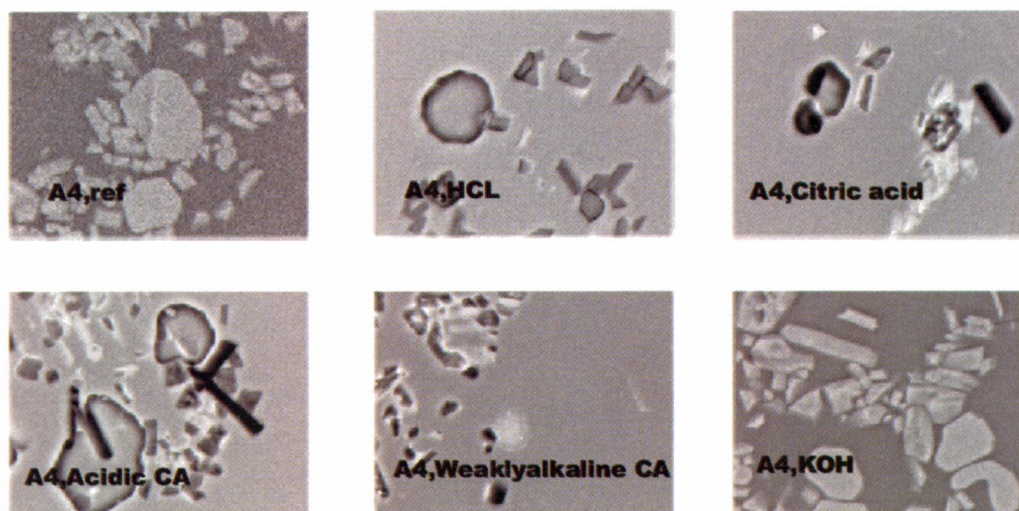
Figure 4. SEM-images of Glaze A4 before and after exposures to different test solutions. CA=cleaning agent
